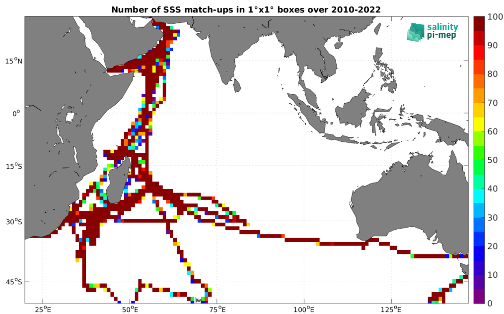
Figure 5: Number of SSS match-ups between TSG (GOSUD-Research-vessel) SSS and the SMOS SSS L4 OI v346 - Weekly (CMEMS-CATDS-LOPS) SSS product for the Indian Ocean Pi-MEP region over 1^\circ \times 1^\circ boxes and for the full satellite product period.
