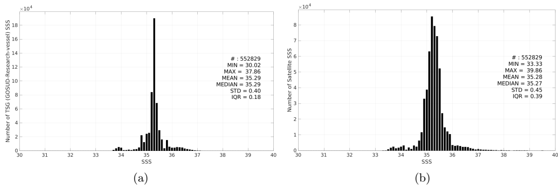
Figure 3: Histograms of SSS from TSG (GOSUD-Research-vessel) (a) and SMOS SSS L4 OI v346 - Weekly (CMEMS-CATDS-LOPS) (b) considering all match-up pairs per bins of 0.1 over the Indian Ocean Pi-MEP region and for the full satellite product period.
