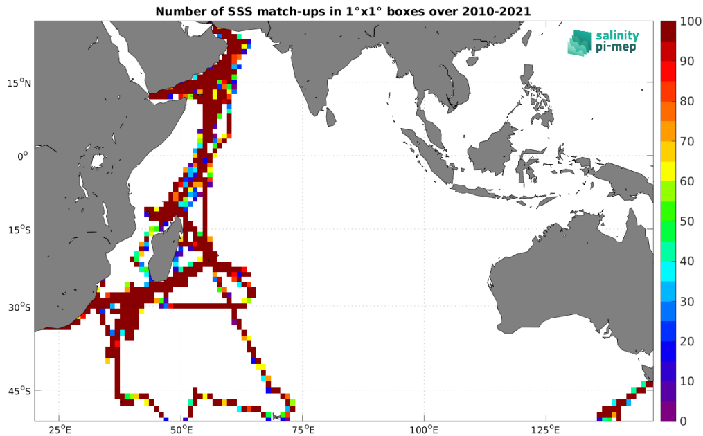
Figure 5: Number of SSS match-ups between TSG (GOSUD-Research-vessel) SSS and the SMOS SSS L4 OI v346 - Weekly (CMEMS-CATDS-LOPS) SSS product for the Indian Ocean Pi-MEP region over 1^\circ \times 1^\circ boxes and for the full satellite product period.
