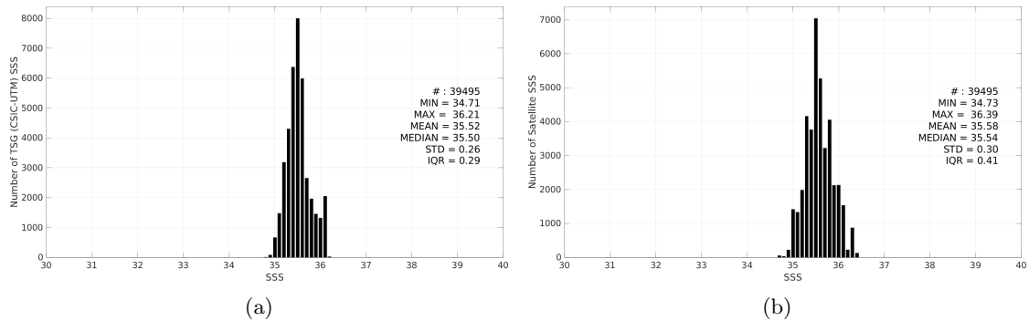
Figure 3: Histograms of SSS from TSG (CSIC-UTM) (a) and SMOS SSS L4 OI v346 - Weekly (CMEMS-CATDS-LOPS) (b) considering all match-up pairs per bins of 0.1 over the Indian Ocean Pi-MEP region and for the full satellite product period.
