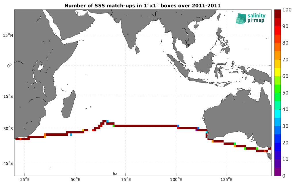
Figure 5: Number of SSS match-ups between TSG (CSIC-UTM) SSS and the SMOS SSS L4 OI v346 - Weekly (CMEMS-CATDS-LOPS) SSS product for the Indian Ocean Pi-MEP region over 1^\circ \times 1^\circ boxes and for the full satellite product period.
