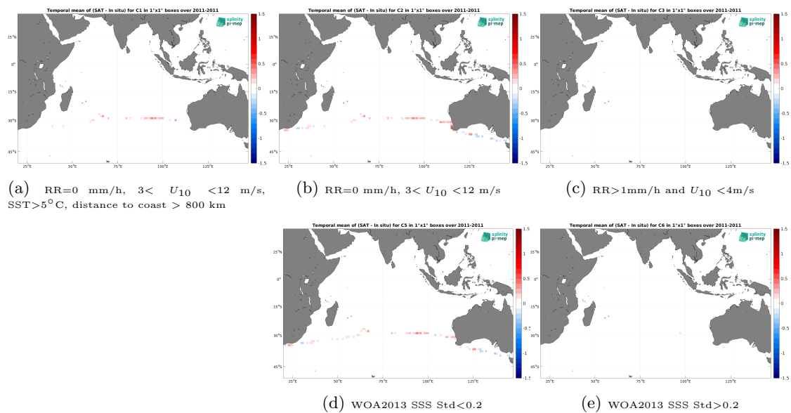
Figure 14: Temporal mean gridded over spatial boxes of size 1^\circ \times 1^\circ of \Delta SSS (SMOS SSS L4 OI v346 - Weekly (CMEMS-CATDS-LOPS) - TSG (CSIC-UTM)) for 5 different subdatasets corresponding to:RR=0 mm/h, 3 < U_{10} < 12 m/s, SST >5^\circ C, distance to coast > 800 km (a), RR=0 mm/h, 3 < U_{10} < 12 m/s (b), RR >1 mm/h and U_{10} < 4 m/s (c), WOA2013 SSS Std <0.2 (d), WOA2013 SSS Std >0.2 (e).
