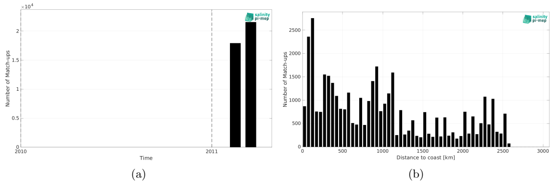
Figure 2: Number of match-ups between TSG (CSIC-UTM) and SMOS SSS L4 OI v346 - Weekly (CMEMS-CATDS-LOPS) SSS as a function of time (a) and as function of the distance to coast (b) over the Indian Ocean Pi-MEP region and for the full satellite product period.
