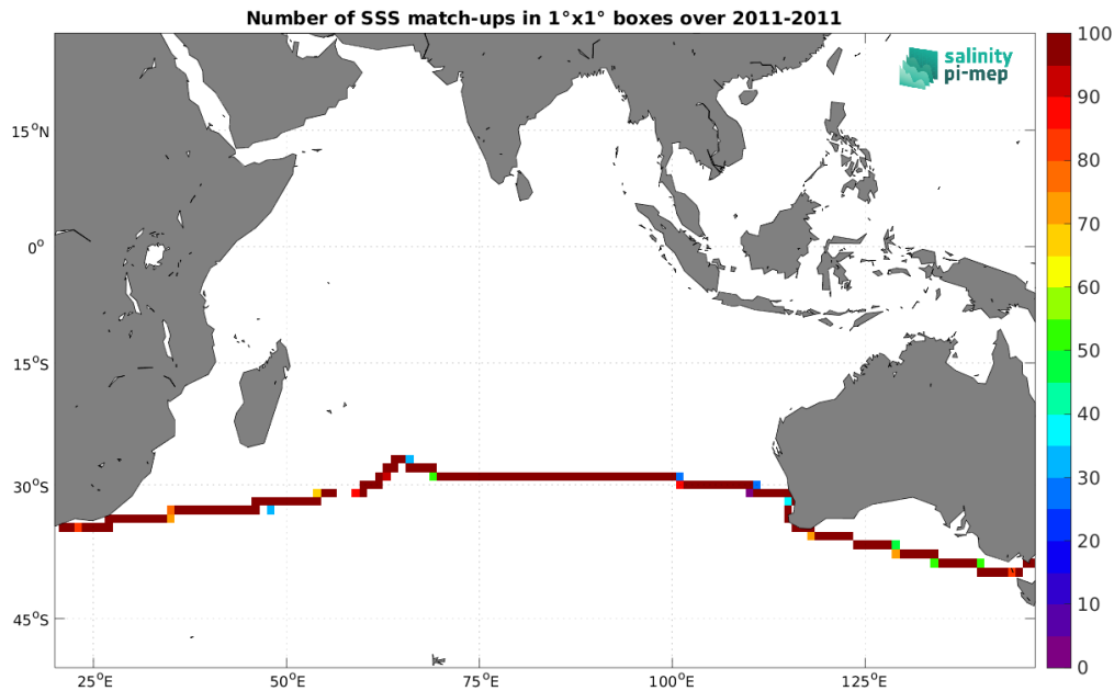
Figure 5: Number of SSS match-ups between TSG (CSIC-UTM) SSS and the SMOS SSS L4 OI v346 - Weekly (CMEMS-CATDS-LOPS) SSS product for the Indian Ocean Pi-MEP region over 1^\circ \times 1^\circ boxes and for the full satellite product period.
