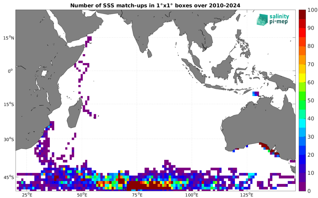
Figure 5: Number of SSS match-ups between Marine mammals SSS and the SMOS SSS L4 OI v346 - Weekly (CMEMS-CATDS-LOPS) SSS product for the Indian Ocean Pi-MEP region over 1^\circ \times 1^\circ boxes and for the full satellite product period.
