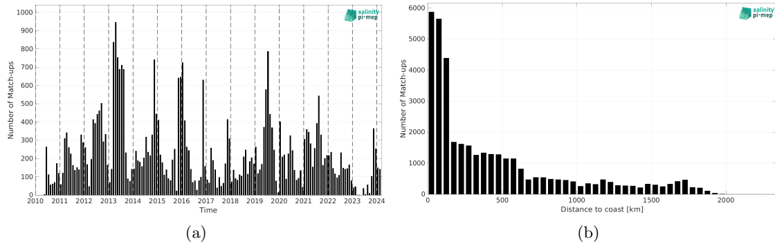
Figure 2: Number of match-ups between Marine mammals and SMOS SSS L4 OI v346 - Weekly (CMEMS-CATDS-LOPS) SSS as a function of time (a) and as function of the distance to coast (b) over the Indian Ocean Pi-MEP region and for the full satellite product period.
