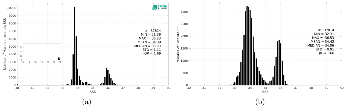
Figure 3: Histograms of SSS from Marine mammals (a) and SMOS SSS L4 OI v346 - Weekly (CMEMS-CATDS-LOPS) (b) considering all match-up pairs per bins of 0.1 over the Indian Ocean Pi-MEP region and for the full satellite product period.
