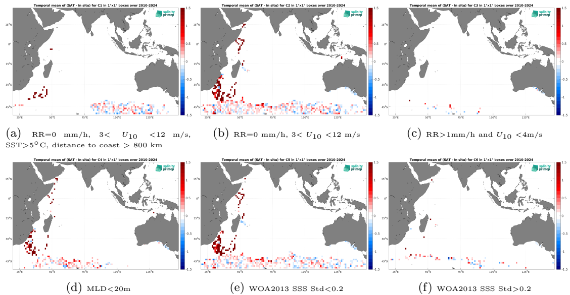
Figure 14: Temporal mean gridded over spatial boxes of size 1^\circ \times 1^\circ of \Delta SSS (SMOS SSS L4 OI v346 - Weekly (CMEMS-CATDS-LOPS) - Marine mammals) for 6 different subdatasets corresponding to:RR=0 mm/h, 3 < U_{10} < 12 m/s, SST>5°C, distance to coast > 800 km (a), RR=0 mm/h, 3 < U_{10} < 12 m/s (b), RR>1mm/h and U_{10} < 4 m/s (c),MLD<20m (d),WOA2013 SSS Std<0.2 (e),WOA2013 SSS Std>0.2 (f).
