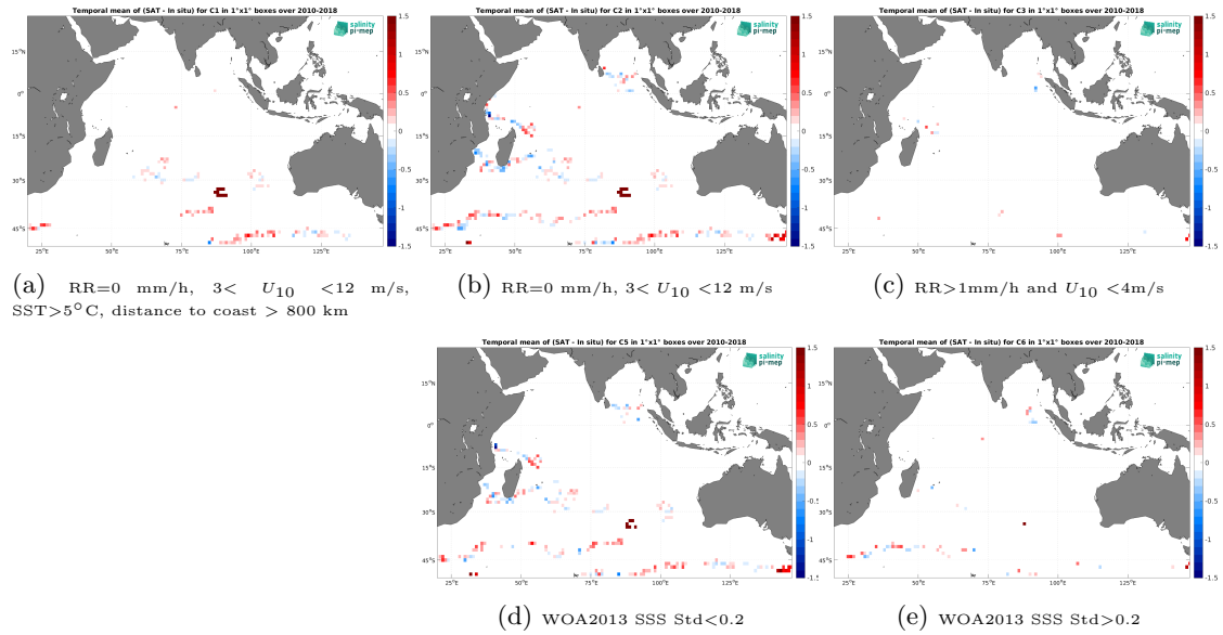
Figure 13: Temporal mean gridded over spatial boxes of size 1^\circ \times 1^\circ of \Delta SSS (SMOS SSS L4 OI v346 - Weekly (CMEMS-CATDS-LOPS) - Surface drifters) for 5 different subdatasets corresponding to:RR=0 mm/h, 3 < U_{10} < 12 m/s, SST >5^\circ C, distance to coast > 800 km (a), RR=0 mm/h, 3 < U_{10} < 12 m/s (b), RR >1 mm/h and U_{10} < 4 m/s (c), WOA2013 SSS Std <0.2 (d), WOA2013 SSS Std >0.2 (e).
