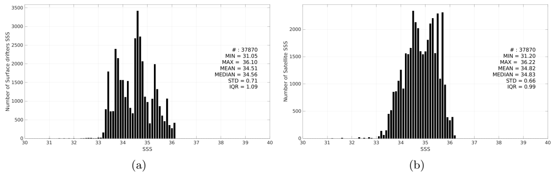
Figure 3: Histograms of SSS from Surface drifters (a) and SMOS SSS L4 OI v346 - Weekly (CMEMS-CATDS-LOPS) (b) considering all match-up pairs per bins of 0.1 over the Indian Ocean Pi-MEP region and for the full satellite product period.
