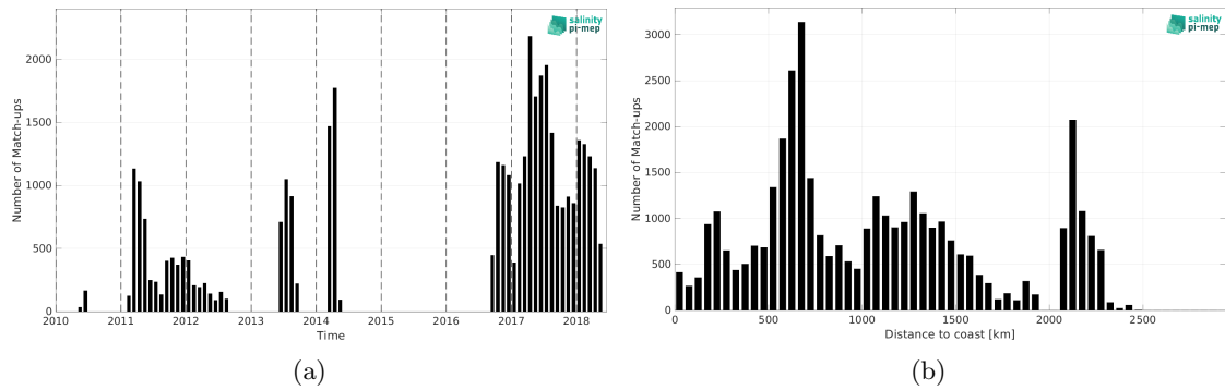
Figure 2: Number of match-ups between Surface drifters and SMOS SSS L4 OI v346 - Weekly (CMEMS-CATDS-LOPS) SSS as a function of time (a) and as function of the distance to coast (b) over the Indian Ocean Pi-MEP region and for the full satellite product period.
