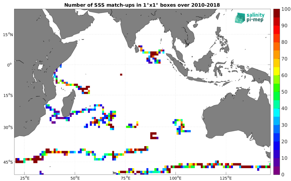
Figure 4: Number of SSS match-ups between Surface drifters SSS and the SMOS SSS L4 OI v346 - Weekly (CMEMS-CATDS-LOPS) SSS product for the Indian Ocean Pi-MEP region over 1^\circ \times 1^\circ boxes and for the full satellite product period.
