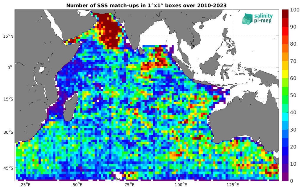
Figure 5: Number of SSS match-ups between Argo SSS and the SMOS SSS L4 OI v346 - Weekly (CMEMS-CATDS-LOPS) SSS product for the Indian Ocean Pi-MEP region over 1^\circ \times 1^\circ boxes and for the full satellite product period.
