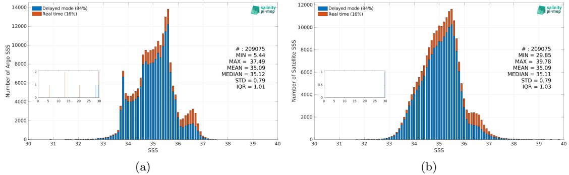
Figure 3: Histograms of SSS from Argo (a) and SMOS SSS L4 OI v346 - Weekly (CMEMS-CATDS-LOPS) (b) considering all match-up pairs per bins of 0.1 over the Indian Ocean Pi-MEP region and for the full satellite product period.
