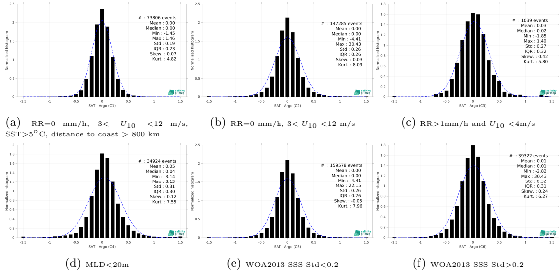
Figure 15: Normalized histogram of \Delta SSS (SMOS SSS L4 OI v346 - Weekly (CMEMS-CATDS-LOPS) - Argo) for 6 different subdatasets corresponding to: RR=0 mm/h, 3 < U_{10} < 12 m/s, SST > 5°C, distance to coast > 800 km (a), RR=0 mm/h, 3 < U_{10} < 12 m/s (b), RR > 1mm/h and U_{10} < 4 m/s (c), MLD < 20m (d), WOA2013 SSS Std < 0.2 (e), WOA2013 SSS Std > 0.2 (f).
