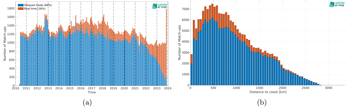
Figure 2: Number of match-ups between Argo and SMOS SSS L4 OI v346 - Weekly (CMEMS-CATDS-LOPS) SSS as a function of time (a) and as function of the distance to coast (b) over the Indian Ocean Pi-MEP region and for the full satellite product period.
