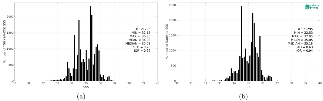
Figure 2: Histograms of SSS from TSG (SAMOS) (a) and SMOS SSS L4 OI v342 - Weekly (CMEMS-CATDS-LOPS) (b) considering all match-up pairs per bins of 0.1 over the Indian Ocean Pi-MEP region and for the full satellite product period.
