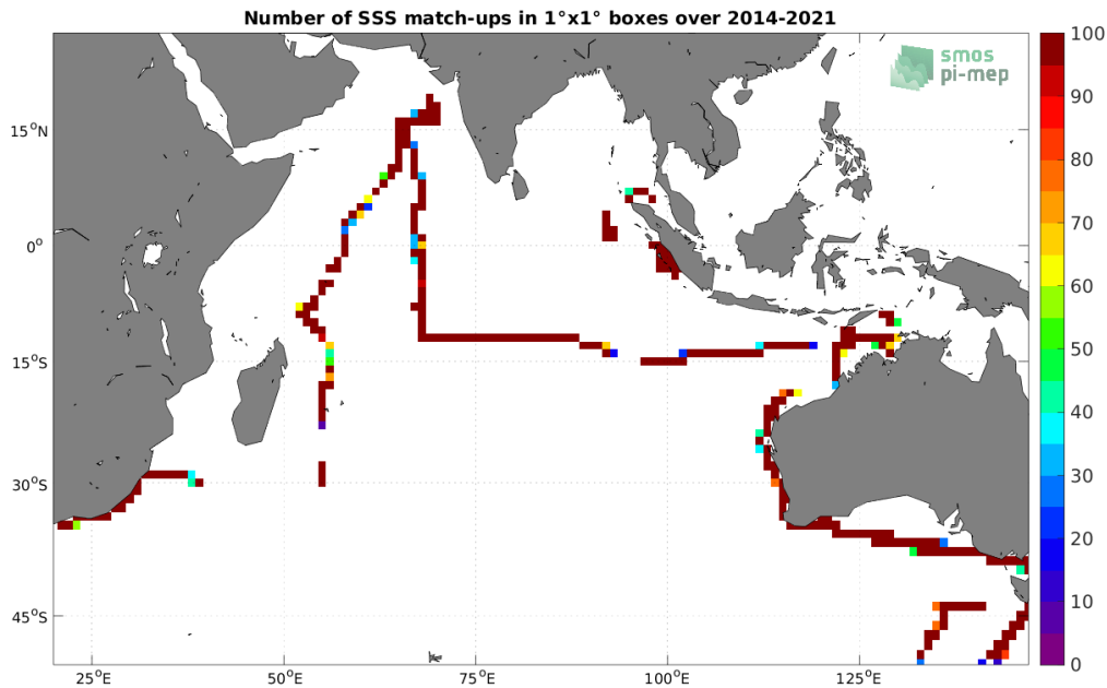
Figure 4: Number of SSS match-ups between TSG (SAMOS) SSS and the SMOS SSS L4 OI v342 - Weekly (CMEMS-CATDS-LOPS) SSS product for the Indian Ocean Pi-MEP region over 1^\circ \times 1^\circ boxes and for the full satellite product period.
