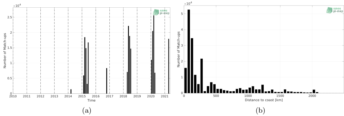
Figure 1: Number of match-ups between TSG (SAMOS) and SMOS SSS L4 OI v342 - Weekly (CMEMS-CATDS-LOPS) SSS as a function of time (a) and as function of the distance to coast (b) over the Indian Ocean Pi-MEP region and for the full satellite product period.
