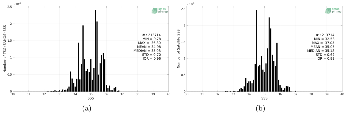
Figure 2: Histograms of SSS from TSG (SAMOS) (a) and SMOS SSS L4 OI v342 - Weekly (CMEMS-CATDS-LOPS) (b) considering all match-up pairs per bins of 0.1 over the Indian Ocean Pi-MEP region and for the full satellite product period.
