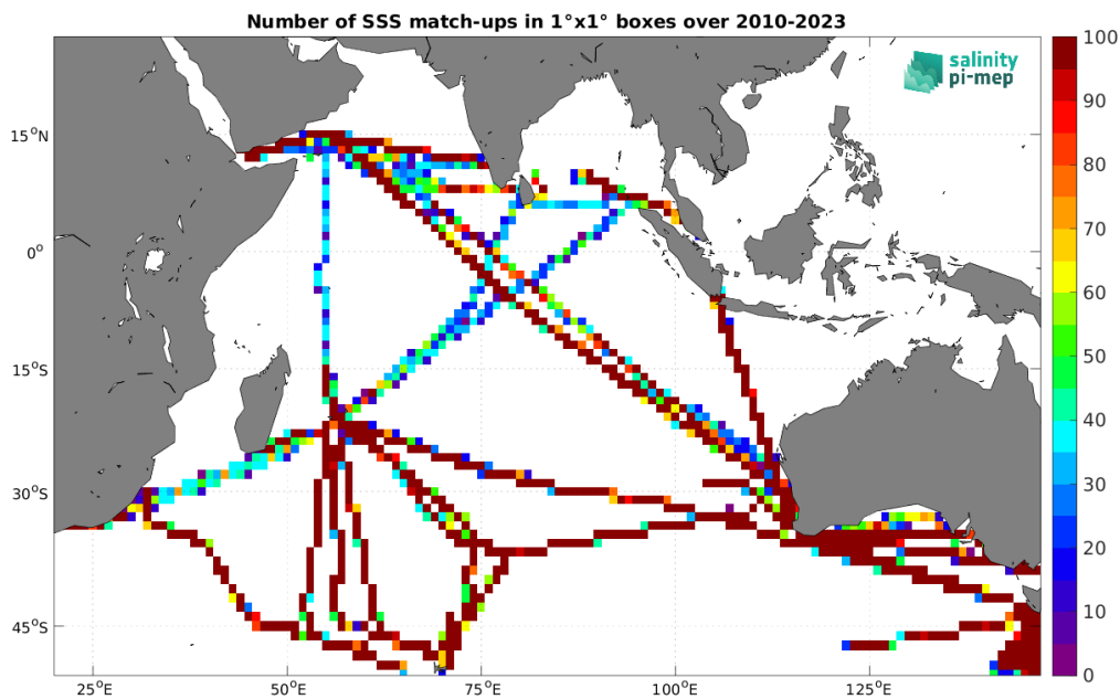
Figure 4: Number of SSS match-ups between TSG (LEGOS-DM) SSS and the SMOS SSS L4 OI v342 - Weekly (CMEMS-CATDS-LOPS) SSS product for the Indian Ocean Pi-MEP region over 1^\circ \times 1^\circ boxes and for the full satellite product period.
