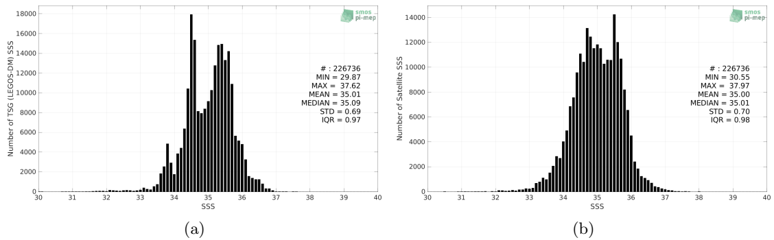
Figure 2: Histograms of SSS from TSG (LEGOS-DM) (a) and SMOS SSS L4 OI v342 - Weekly (CMEMS-CATDS-LOPS) (b) considering all match-up pairs per bins of 0.1 over the Indian Ocean Pi-MEP region and for the full satellite product period.
