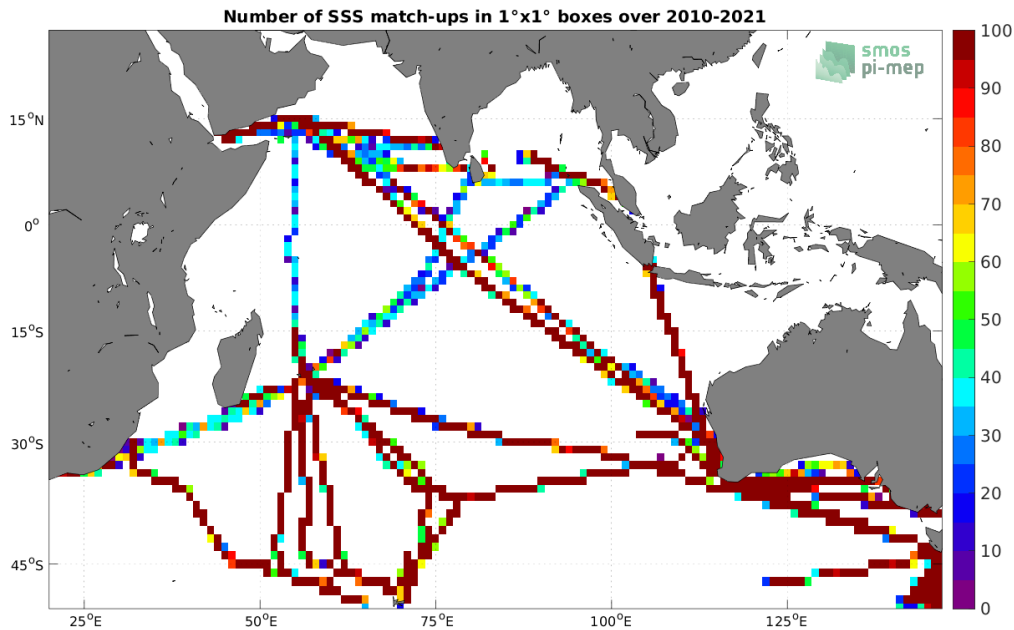
Figure 4: Number of SSS match-ups between TSG (LEGOS-DM) SSS and the SMOS SSS L4 OI v342 - Weekly (CMEMS-CATDS-LOPS) SSS product for the Indian Ocean Pi-MEP region over 1^\circ \times 1^\circ boxes and for the full satellite product period.
