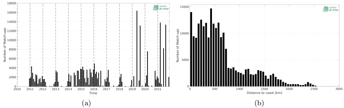
Figure 1: Number of match-ups between TSG (LEGOS-DM) and SMOS SSS L4 OI v342 - Weekly (CMEMS-CATDS-LOPS) SSS as a function of time (a) and as function of the distance to coast (b) over the Indian Ocean Pi-MEP region and for the full satellite product period.
