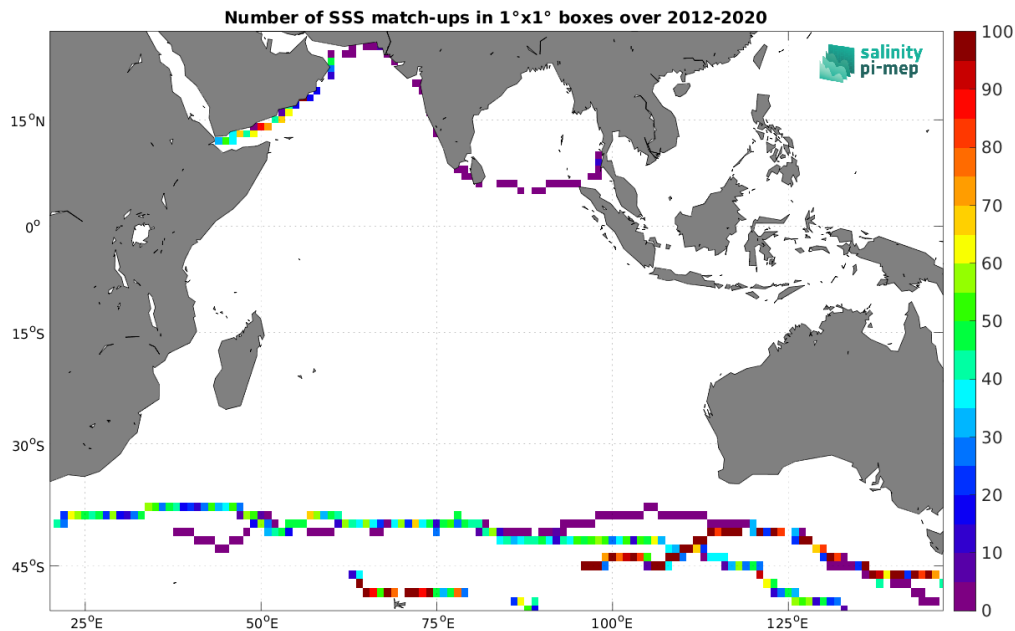
Figure 4: Number of SSS match-ups between TSG (GOSUD-Sailing-ship) SSS and the SMOS SSS L4 OI v342 - Weekly (CMEMS-CATDS-LOPS) SSS product for the Indian Ocean Pi-MEP region over 1^\circ \times 1^\circ boxes and for the full satellite product period.
