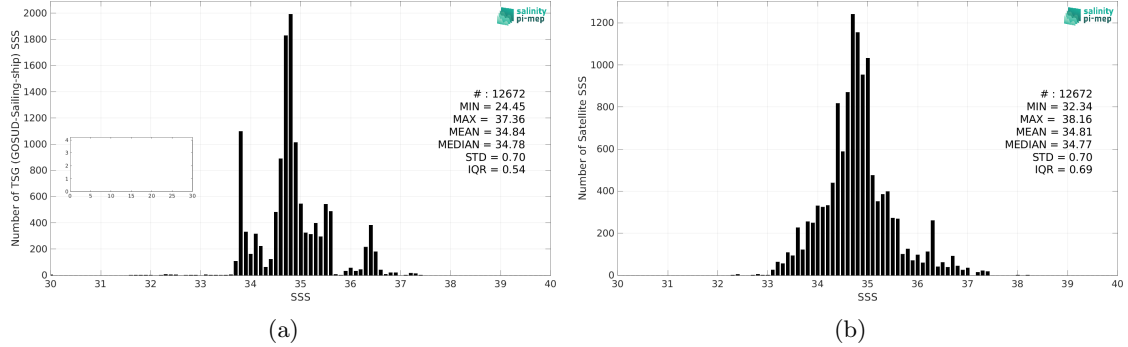
Figure 2: Histograms of SSS from TSG (GOSUD-Sailing-ship) (a) and SMOS SSS L4 OI v342 - Weekly (CMEMS-CATDS-LOPS) (b) considering all match-up pairs per bins of 0.1 over the Indian Ocean Pi-MEP region and for the full satellite product period.
