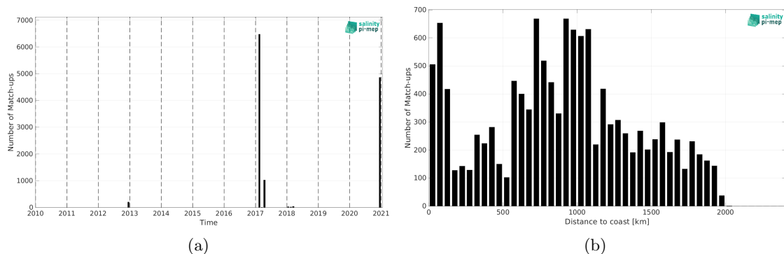
Figure 1: Number of match-ups between TSG (GOSUD-Sailing-ship) and SMOS SSS L4 OI v342 - Weekly (CMEMS-CATDS-LOPS) SSS as a function of time (a) and as function of the distance to coast (b) over the Indian Ocean Pi-MEP region and for the full satellite product period.
