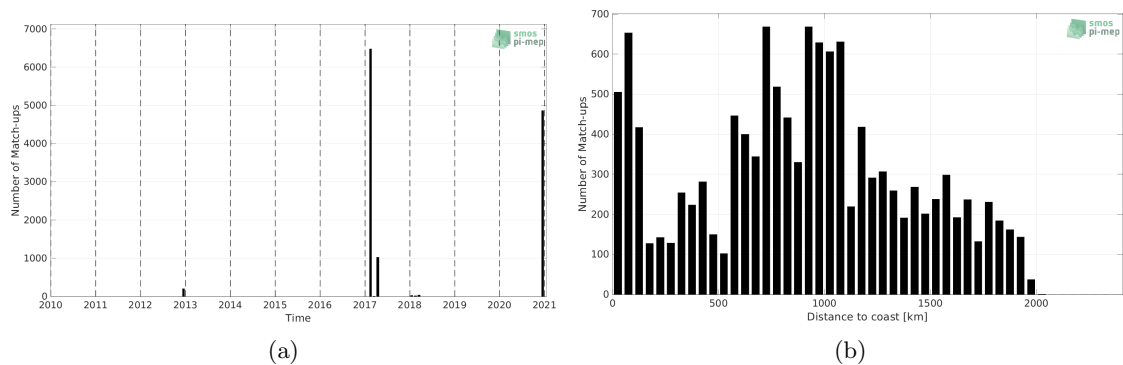
Figure 1: Number of match-ups between TSG (GOSUD-Sailing-ship) and SMOS SSS L4 OI v342 - Weekly (CMEMS-CATDS-LOPS) SSS as a function of time (a) and as function of the distance to coast (b) over the Indian Ocean Pi-MEP region and for the full satellite product period.
