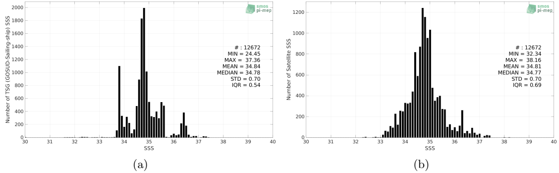
Figure 2: Histograms of SSS from TSG (GOSUD-Sailing-ship) (a) and SMOS SSS L4 OI v342 - Weekly (CMEMS-CATDS-LOPS) (b) considering all match-up pairs per bins of 0.1 over the Indian Ocean Pi-MEP region and for the full satellite product period.
