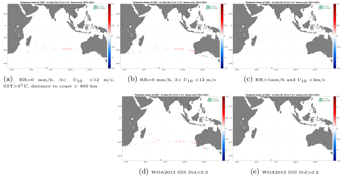
Figure 12: Temporal mean gridded over spatial boxes of size 1^{\circ}\times 1^{\circ} of \Delta\text{SSS} (SMOS SSS L4 OI v342 - Weekly (CMEMS-CATDS-LOPS) - TSG (CSIC-UTM)) for 5 different subdatasets corresponding to:RR=0 mm/h, 3 < U_{10} < 12 m/s, SST >5^{\circ}\text{C} , distance to coast > 800 km (a), RR=0 mm/h, 3 < U_{10} < 12 m/s (b), RR >1 mm/h and U_{10} < 4 m/s (c), WOA2013 SSS Std <0.2 (d), WOA2013 SSS Std >0.2 (e).
