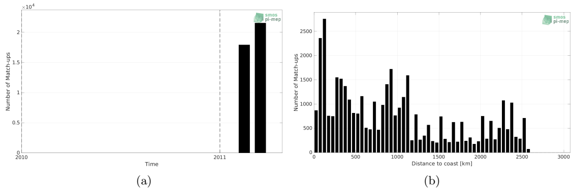
Figure 1: Number of match-ups between TSG (CSIC-UTM) and SMOS SSS L4 OI v342 - Weekly (CMEMS-CATDS-LOPS) SSS as a function of time (a) and as function of the distance to coast (b) over the Indian Ocean Pi-MEP region and for the full satellite product period.
