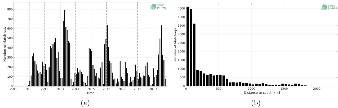
Figure 1: Number of match-ups between Marine mammals and SMOS SSS L4 OI v342 - Weekly (CMEMS-CATDS-LOPS) SSS as a function of time (a) and as function of the distance to coast (b) over the Indian Ocean Pi-MEP region and for the full satellite product period.
