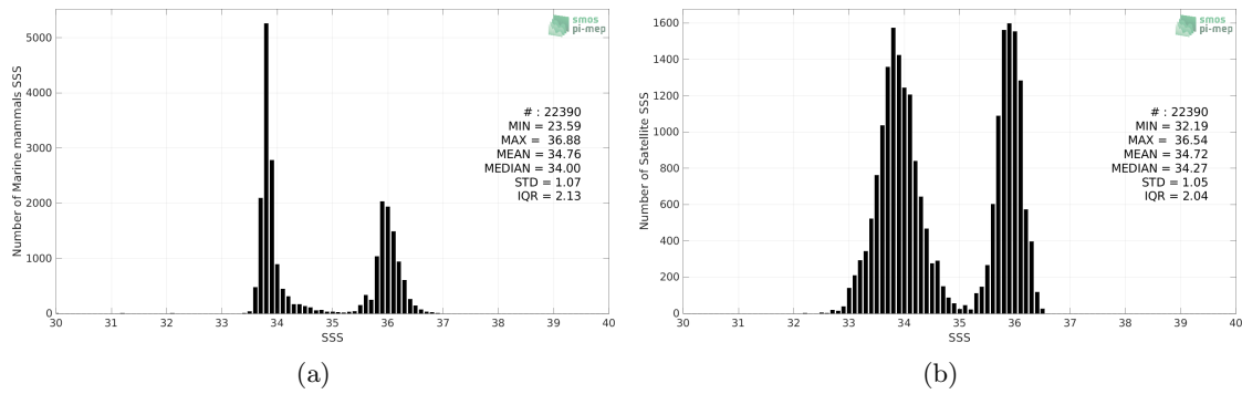
Figure 2: Histograms of SSS from Marine mammals (a) and SMOS SSS L4 OI v342 - Weekly (CMEMS-CATDS-LOPS) (b) considering all match-up pairs per bins of 0.1 over the Indian Ocean Pi-MEP region and for the full satellite product period.
