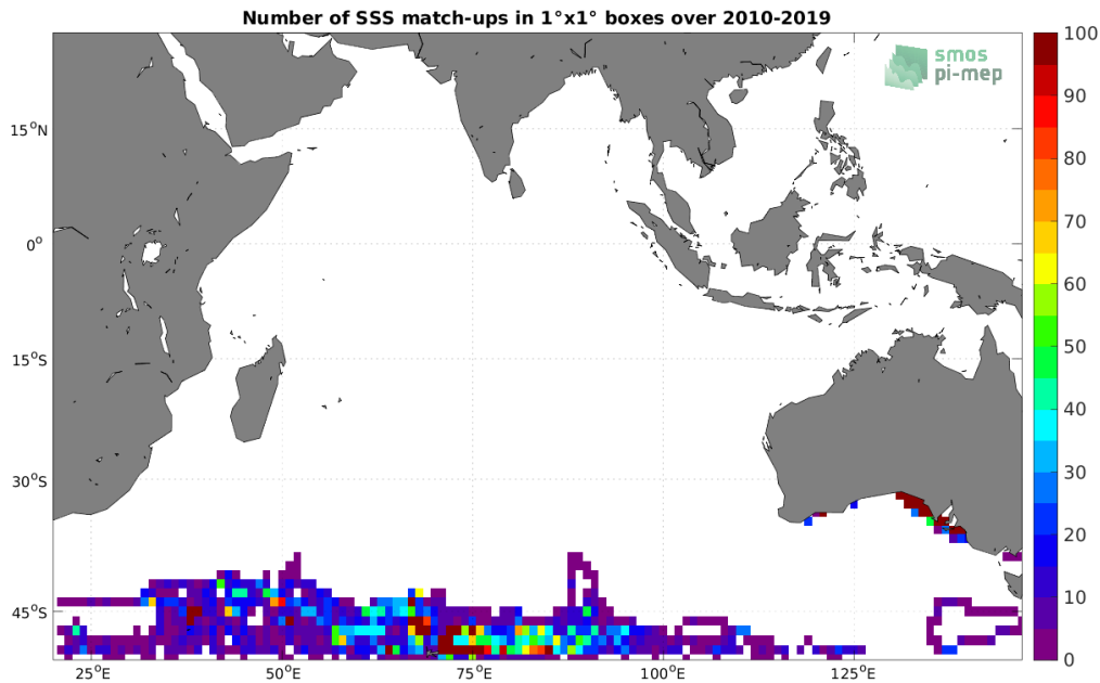
Figure 4: Number of SSS match-ups between Marine mammals SSS and the SMOS SSS L4 OI v342 - Weekly (CMEMS-CATDS-LOPS) SSS product for the Indian Ocean Pi-MEP region over 1^\circ \times 1^\circ boxes and for the full satellite product period.
