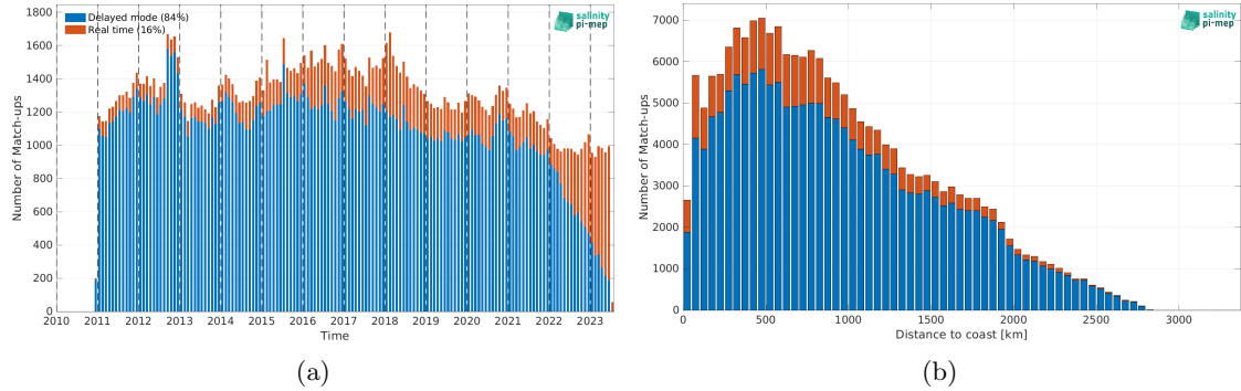
Figure 1: Number of match-ups between Argo and SMOS SSS L4 OI v342 - Weekly (CMEMS-CATDS-LOPS) SSS as a function of time (a) and as function of the distance to coast (b) over the Indian Ocean Pi-MEP region and for the full satellite product period.
