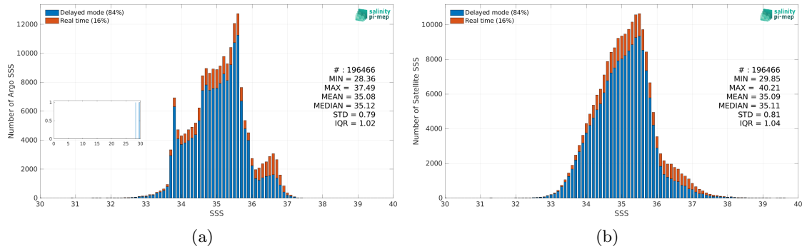
Figure 2: Histograms of SSS from Argo (a) and SMOS SSS L4 OI v342 - Weekly (CMEMS-CATDS-LOPS) (b) considering all match-up pairs per bins of 0.1 over the Indian Ocean Pi-MEP region and for the full satellite product period.
