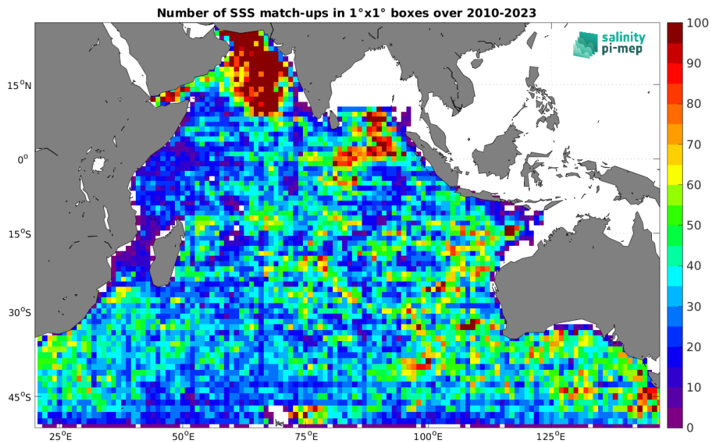
Figure 4: Number of SSS match-ups between Argo SSS and the SMOS SSS L4 OI v342 - Weekly (CMEMS-CATDS-LOPS) SSS product for the Indian Ocean Pi-MEP region over 1^\circ \times 1^\circ boxes and for the full satellite product period.
