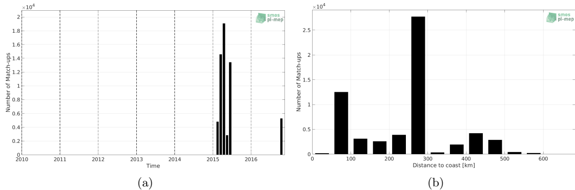
Figure 1: Number of match-ups between TSG (SAMOS) and SMOS L4 v2 Weekly (CATDS-CECOS-IFREMER) SSS as a function of time (a) and as function of the distance to coast (b) over the Indian Ocean Pi-MEP region and for the full satellite product period.
