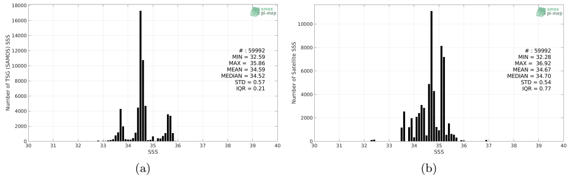
Figure 2: Histograms of SSS from TSG (SAMOS) (a) and SMOS L4 v2 Weekly (CATDS-CECOS-IFREMER) (b) considering all match-up pairs per bins of 0.1 over the Indian Ocean Pi-MEP region and for the full satellite product period.
