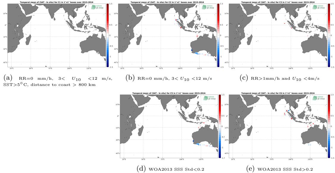
Figure 12: Temporal mean gridded over spatial boxes of size 1^{\circ}\times 1^{\circ} of \Delta\text{SSS} (SMOS L4 v2 Weekly (CATDS-CECOS-IFREMER) - TSG (SAMOS)) for 5 different subdatasets corresponding to:RR=0 mm/h, 3 < U_{10} < 12 m/s, SST >5^{\circ}\text{C} , distance to coast > 800 km (a), RR=0 mm/h, 3 < U_{10} < 12 m/s (b), RR >1 mm/h and U_{10} < 4 m/s (c), WOA2013 SSS Std <0.2 (d), WOA2013 SSS Std >0.2 (e).
