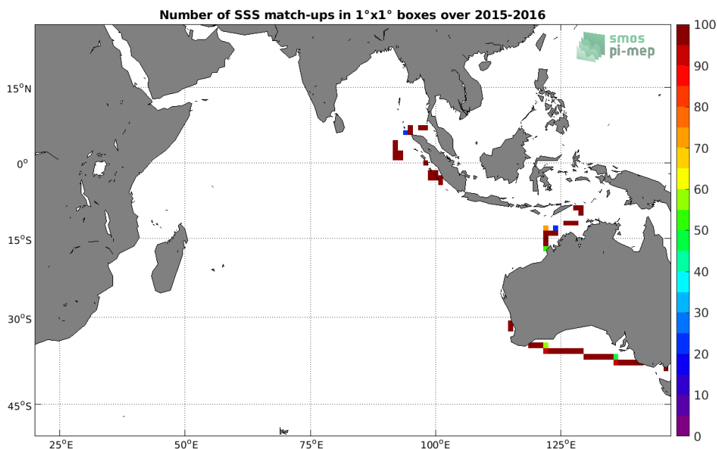
Figure 4: Number of SSS match-ups between TSG (SAMOS) SSS and the SMOS L4 v2 Weekly (CATDS-CECOS-IFREMER) SSS product for the Indian Ocean Pi-MEP region over 1°x1° boxes and for the full satellite product period.
