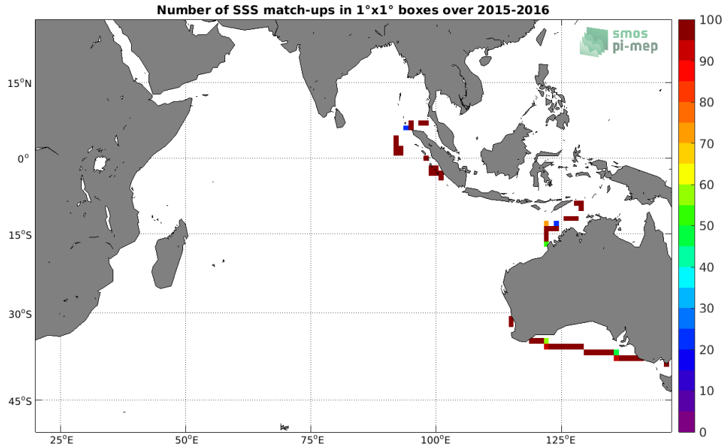
Figure 4: Number of SSS match-ups between TSG (SAMOS) SSS and the SMOS L4 v2 Weekly (CATDS-CECOS-IFREMER) SSS product for the Indian Ocean Pi-MEP region over 1°x1° boxes and for the full satellite product period.
