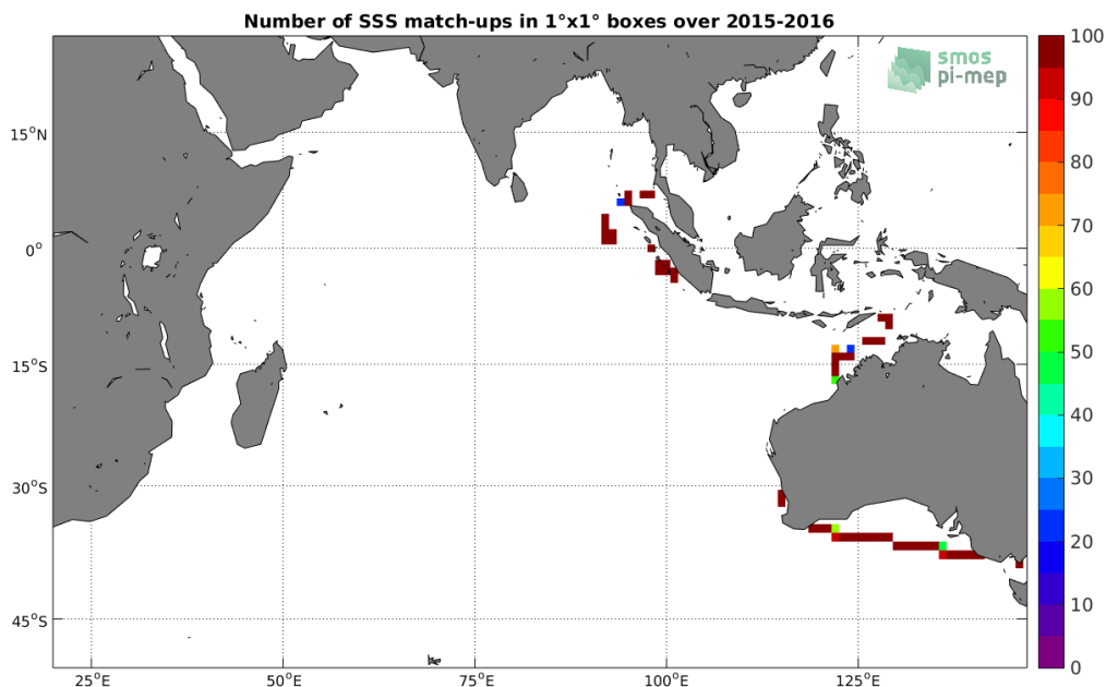
Figure 4: Number of SSS match-ups between TSG-SAMOS SSS and the SMOS-L4-CATDS-CECOS-IFREMER-V2-WEEKLY-0.5DEG SSS product for the Indian Ocean Pi-MEP region over 1°x1° boxes and for the full satellite product period.
