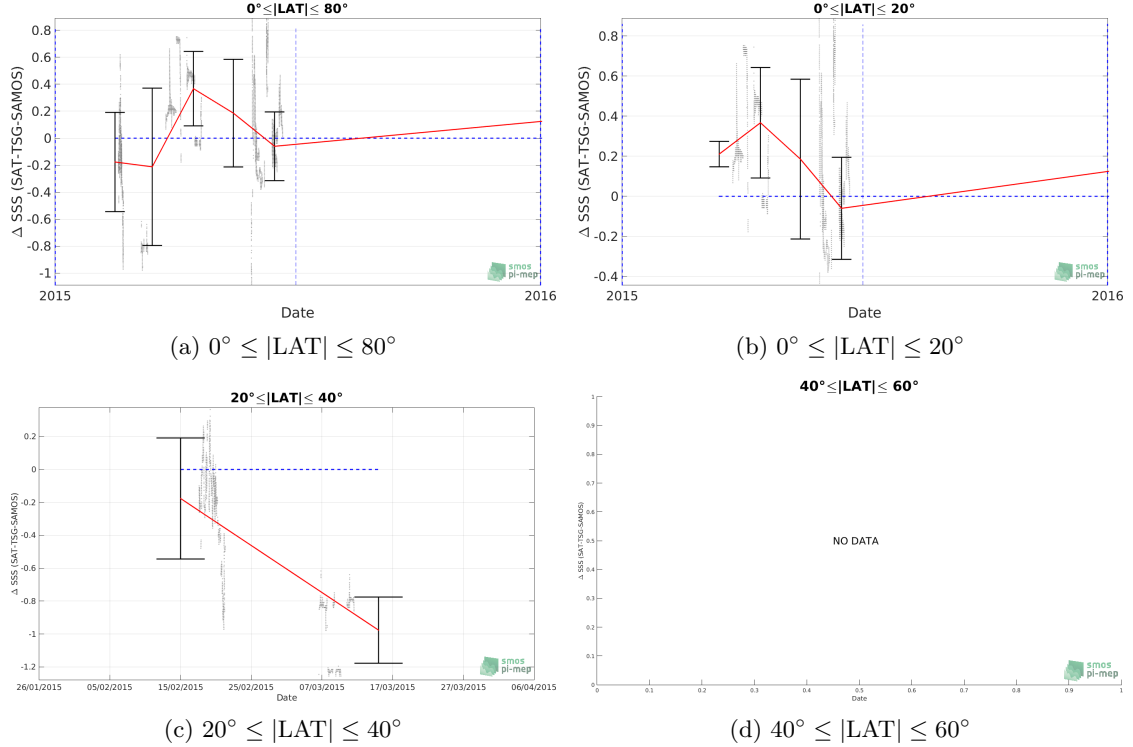
Figure 10: Monthly-averaged mean (red curves) \Delta SSS (Satellite - TSG-SAMOS) and \pm 1 Std (black vertical thick bars) as function of time for all the collected Pi-MEP match-up pairs estimated over the Indian Ocean Pi-MEP region and for the full satellite product period are shown for different latitude bands: (a) Latitude band 80°S-80°N, (b) latitude band 20°S-20°N, (c) Mid Latitude bands 40°S-20°S and 20°N-40°N and (d) Latitude bands 60°S-40°S and 40°N-60°N.
