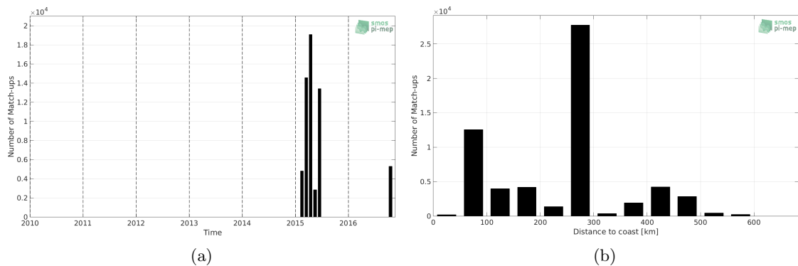
Figure 1: Number of match-ups between TSG-SAMOS and SMOS-L4-CATDS-CECOS-IFREMER-V2-WEEKLY-0.5DEG SSS as a function of time (a) and as function of the distance to coast (b) over the Indian Ocean Pi-MEP region and for the full satellite product period.
