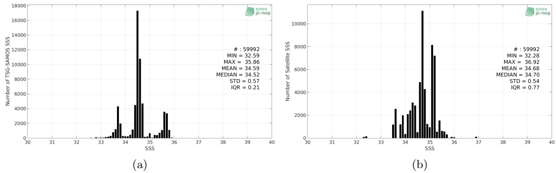
Figure 2: Histograms of SSS from TSG-SAMOS (a) and SMOS-L4-CATDS-CECOS-IFREMER-V2-WEEKLY-0.5DEG (b) considering all match-up pairs per bins of 0.1 over the Indian Ocean Pi-MEP region and for the full satellite product period.
