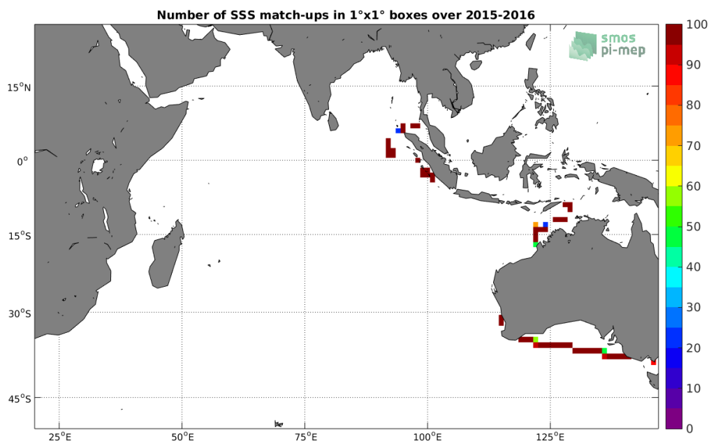
Figure 4: Number of SSS match-ups between TSG-SAMOS SSS and the SMOS-L4-CATDS-CECOS-IFREMER-V2-WEEKLY-0.5DEG SSS product for the Indian Ocean Pi-MEP region over 1°x1° boxes and for the full satellite product period.
