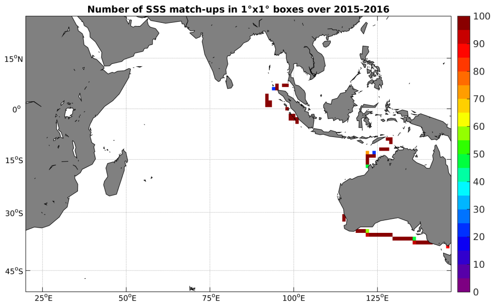
Figure 4: Number of SSS match-ups between TSG-SAMOS SSS and the SMOS-L4-CATDS-CECOS-IFREMER-V2-WEEKLY-0.5DEG SSS product for the Indian Ocean Pi-MEP region over 1^\circ \times 1^\circ boxes and for the full satellite product period.
