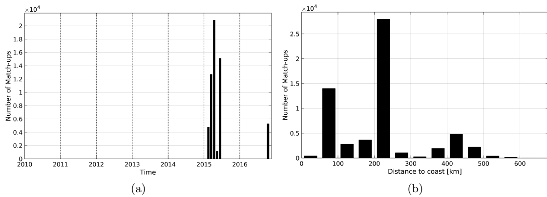
Figure 1: Number of match-ups between TSG-SAMOS and SMOS-L4-CATDS-CECOS-IFREMER-V2-WEEKLY-0.5DEG SSS as a function of time (a) and as function of the distance to coast (b) over the Indian Ocean Pi-MEP region and for the full satellite product period.
