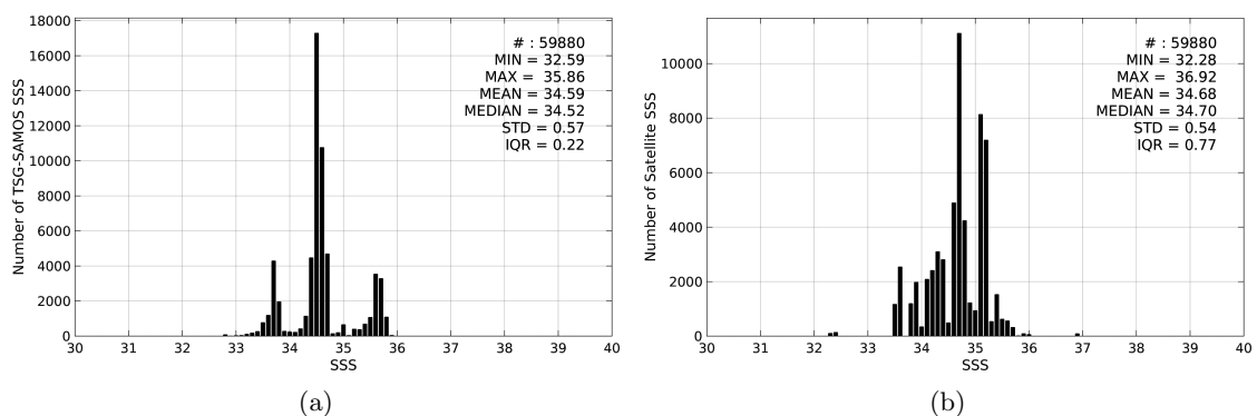
Figure 2: Histograms of SSS from TSG-SAMOS (a) and SMOS-L4-CATDS-CECOS-IFREMER-V2-WEEKLY-0.5DEG (b) considering all match-up pairs per bins of 0.1 over the Indian Ocean Pi-MEP region and for the full satellite product period.
