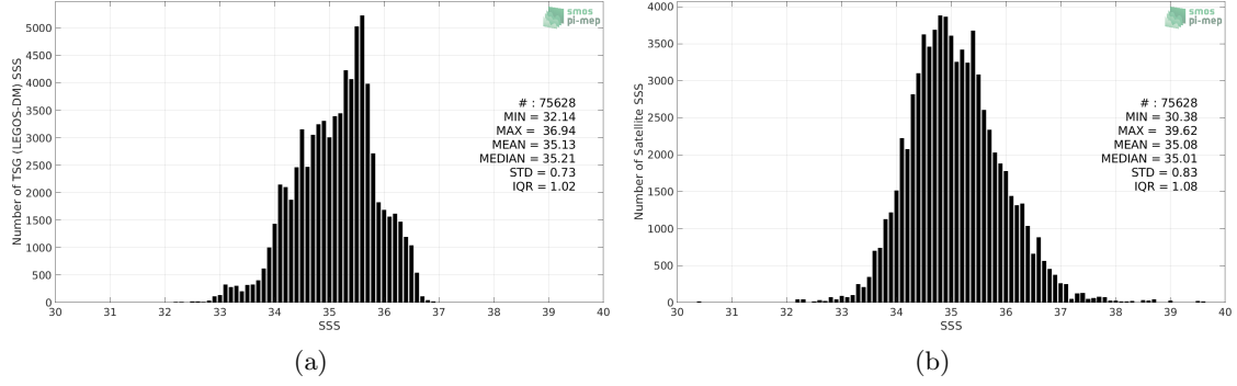
Figure 2: Histograms of SSS from TSG (LEGOS-DM) (a) and SMOS L4 v2 Weekly (CATDS-CECOS-IFREMER) (b) considering all match-up pairs per bins of 0.1 over the Indian Ocean Pi-MEP region and for the full satellite product period.
