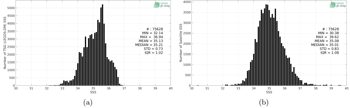
Figure 2: Histograms of SSS from TSG (LEGOS-DM) (a) and SMOS L4 v2 Weekly (CATDS-CECOS-IFREMER) (b) considering all match-up pairs per bins of 0.1 over the Indian Ocean Pi-MEP region and for the full satellite product period.
