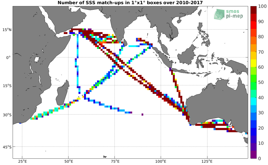
Figure 4: Number of SSS match-ups between TSG (LEGOS-DM) SSS and the SMOS L4 v2 Weekly (CATDS-CECOS-IFREMER) SSS product for the Indian Ocean Pi-MEP region over 1^\circ \times 1^\circ boxes and for the full satellite product period.
