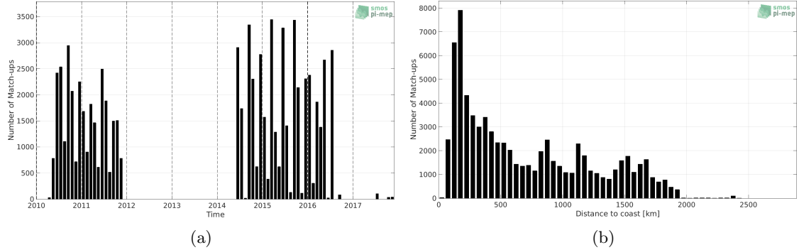
Figure 1: Number of match-ups between TSG (LEGOS-DM) and SMOS L4 v2 Weekly (CATDS-CECOS-IFREMER) SSS as a function of time (a) and as function of the distance to coast (b) over the Indian Ocean Pi-MEP region and for the full satellite product period.
