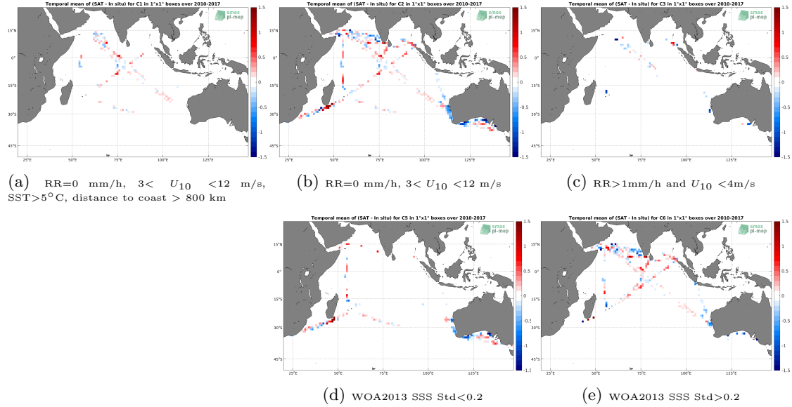
Figure 12: Temporal mean gridded over spatial boxes of size 1^{\circ}\times 1^{\circ} of \Delta\text{SSS} (SMOS L4 v2 Weekly (CATDS-CECOS-IFREMER) - TSG (LEGOS-DM)) for 5 different subdatasets corresponding to:RR=0 mm/h, 3 < U_{10} < 12 m/s, SST >5^{\circ}\text{C} , distance to coast > 800 km (a), RR=0 mm/h, 3 < U_{10} < 12 m/s (b), RR >1 mm/h and U_{10} < 4 m/s (c), WOA2013 SSS Std <0.2 (d), WOA2013 SSS Std >0.2 (e).
