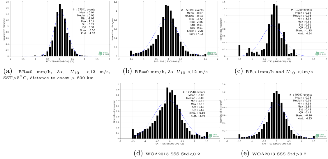
Figure 13: Normalized histogram of \Delta\text{SSS} (SMOS L4 v2 Weekly (CATDS-CECOS-IFREMER) - TSG (LEGOS-DM)) for 5 different subdatasets corresponding to: RR=0 mm/h, 3 < U_{10} < 12 m/s, SST > 5^\circ\text{C} , distance to coast > 800 km (a), RR=0 mm/h, 3 < U_{10} < 12 m/s (b), RR > 1\text{mm/h} and U_{10} < 4\text{m/s} (c), WOA2013 SSS Std < 0.2 (d), WOA2013 SSS Std > 0.2 (e).
