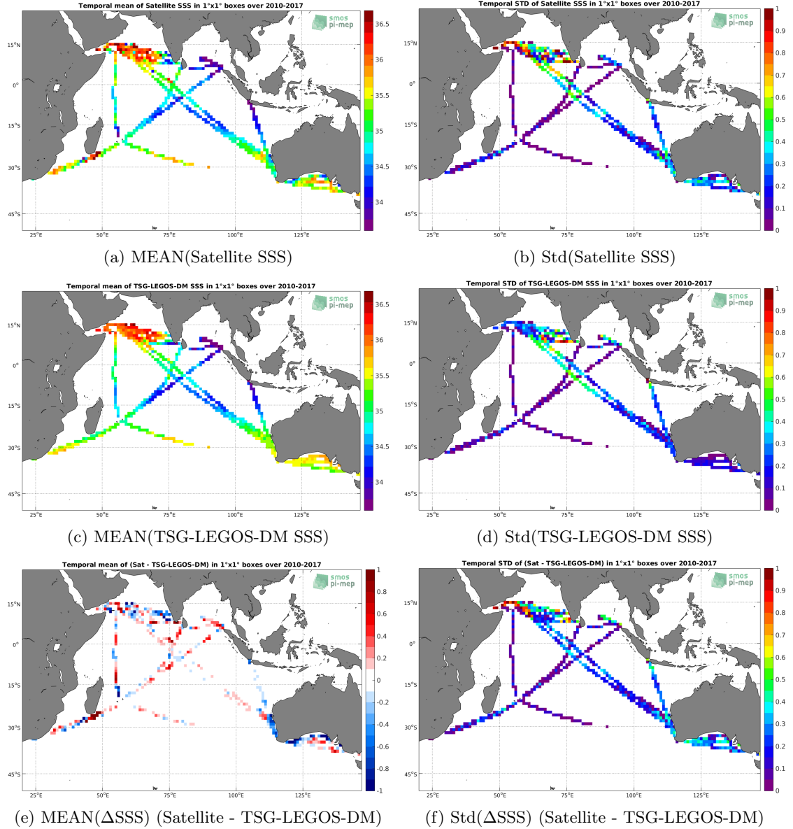
Figure 6: Temporal mean (left) and Std (right) of SSS from SMOS-L4-CATDS-CECOS-IFREMER-V2-WEEKLY-0.5DEG (top), TSG-LEGOS-DM (middle), and of \Delta SSS (Satellite - TSG-LEGOS-DM). Only match-up pairs are used to generate these maps.
