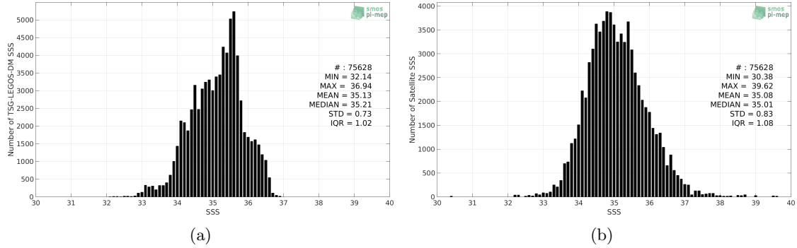
Figure 2: Histograms of SSS from TSG-LEGOS-DM (a) and SMOS-L4-CATDS-CECOS-IFREMER-V2-WEEKLY-0.5DEG (b) considering all match-up pairs per bins of 0.1 over the Indian Ocean Pi-MEP region and for the full satellite product period.
