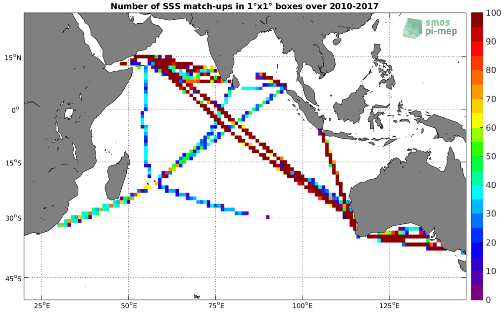
Figure 4: Number of SSS match-ups between TSG-LEGOS-DM SSS and the SMOS-L4-CATDS-CECOS-IFREMER-V2-WEEKLY-0.5DEG SSS product for the Indian Ocean Pi-MEP region over 1°x1° boxes and for the full satellite product period.
