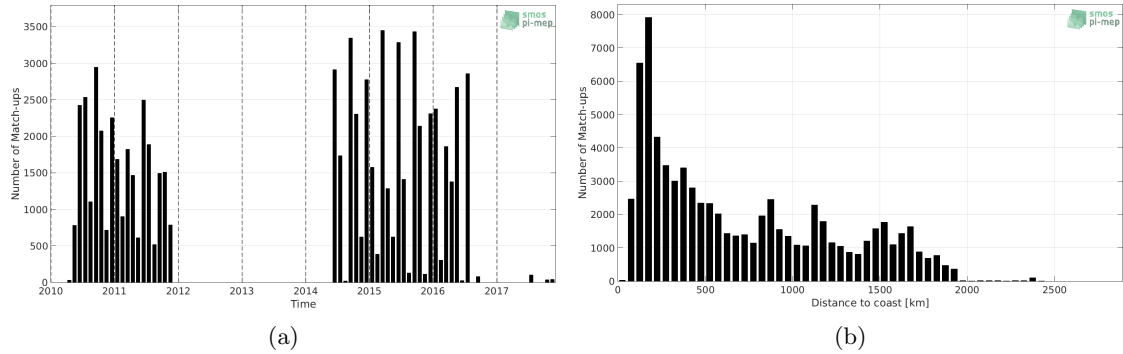
Figure 1: Number of match-ups between TSG-LEGOS-DM and SMOS-L4-CATDS-CECOS-IFREMER-V2-WEEKLY-0.5DEG SSS as a function of time (a) and as function of the distance to coast (b) over the Indian Ocean Pi-MEP region and for the full satellite product period.
