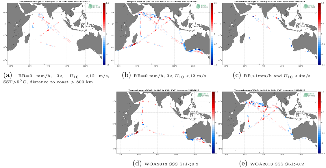
Figure 12: Temporal mean gridded over spatial boxes of size 1^{\circ}\times 1^{\circ} of \Delta\text{SSS} (SMOS-L4-CATDS-CECOS-IFREMER-V2-WEEKLY-0.5DEG - TSG-LEGOS-DM) for 5 different subdatasets corresponding to: \text{RR}=0 mm/h, 3 < U_{10} < 12 m/s, \text{SST} > 5^{\circ}\text{C} , distance to coast > 800 km (a), \text{RR}=0 mm/h, 3 < U_{10} < 12 m/s (b), \text{RR} > 1 mm/h and U_{10} < 4 m/s (c), WOA2013 SSS Std < 0.2 (d), WOA2013 SSS Std > 0.2 (e).
