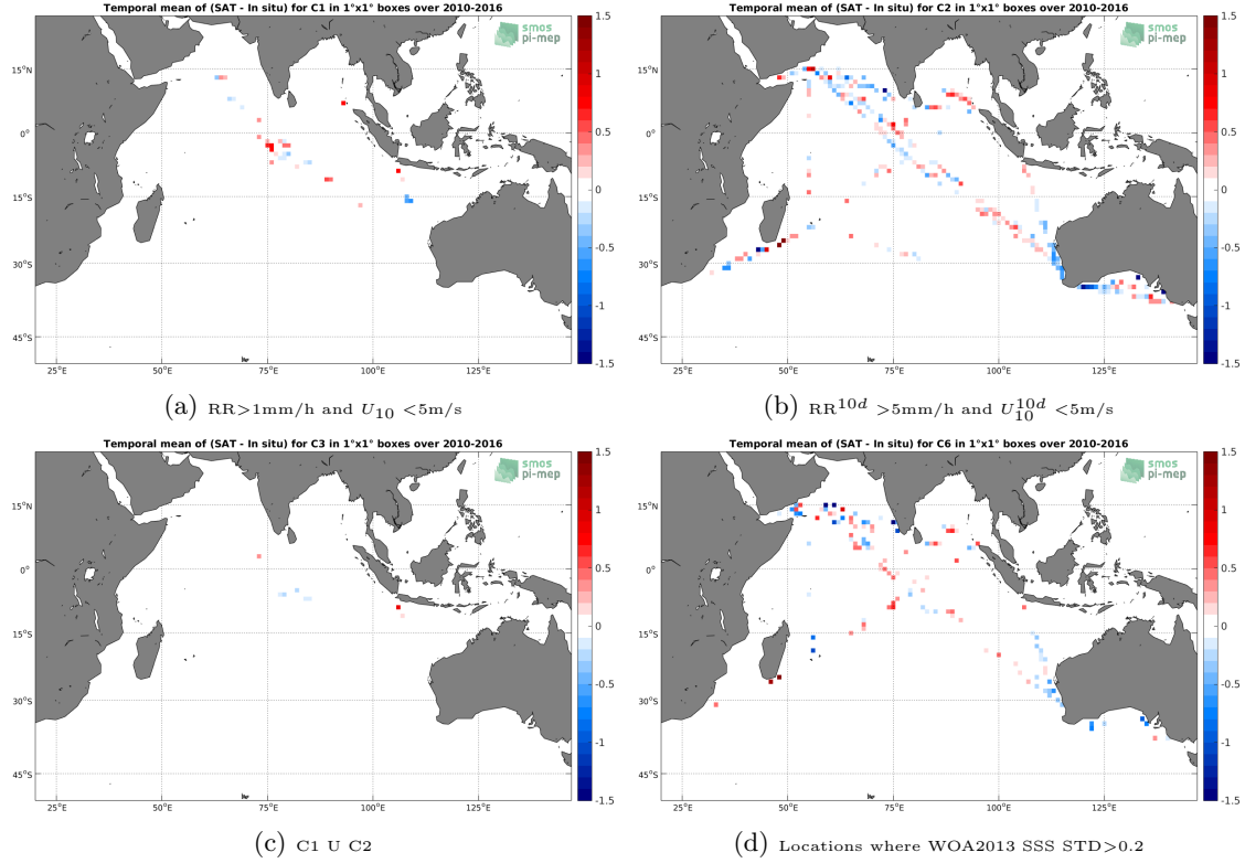
Figure 12: Temporal mean gridded over spatial boxes of size 1^\circ \times 1^\circ of \Delta SSS (SMOS-L4-CATDS-CECOS-IFREMER-V2-WEEKLY-0.5DEG - TSG-LEGOS-DM) for 4 different subdatasets corresponding to: RR > 1\text{mm/h} and U_{10} < 5\text{m/s} (a), RR^{10d} > 5\text{mm/h} and U_{10}^{10d} < 5\text{m/s} (b), C1 U C2 (c), Locations where WOA2013 SSS STD > 0.2 (d).
