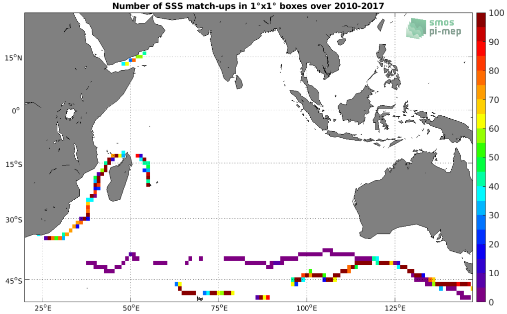
Figure 4: Number of SSS match-ups between TSG (GOSUD-Sailing-ship) SSS and the SMOS L4 v2 Weekly (CATDS-CECOS-IFREMER) SSS product for the Indian Ocean Pi-MEP region over 1^\circ \times 1^\circ boxes and for the full satellite product period.
