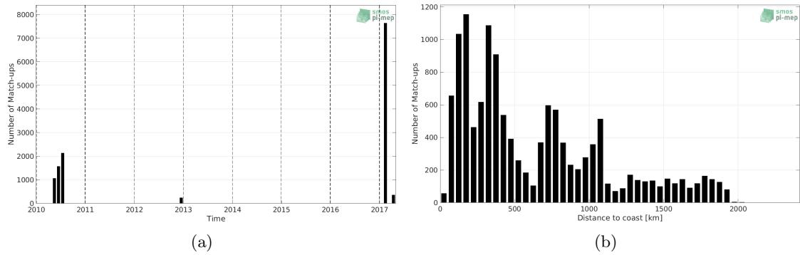
Figure 1: Number of match-ups between TSG (GOSUD-Sailing-ship) and SMOS L4 v2 Weekly (CATDS-CECOS-IFREMER) SSS as a function of time (a) and as function of the distance to coast (b) over the Indian Ocean Pi-MEP region and for the full satellite product period.
