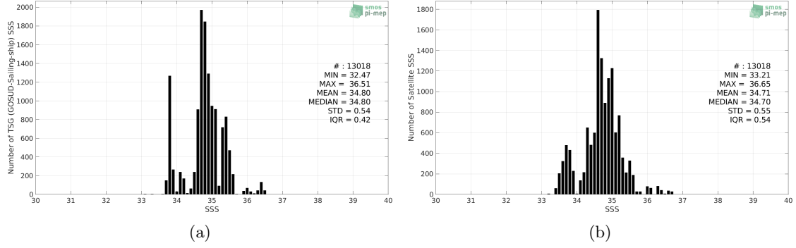
Figure 2: Histograms of SSS from TSG (GOSUD-Sailing-ship) (a) and SMOS L4 v2 Weekly (CATDS-CECOS-IFREMER) (b) considering all match-up pairs per bins of 0.1 over the Indian Ocean Pi-MEP region and for the full satellite product period.
