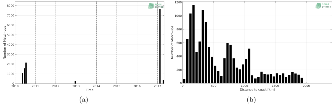
Figure 1: Number of match-ups between TSG-GOSUD-Sailing-ship and SMOS-L4-CATDS-CECOS-IFREMER-V2-WEEKLY-0.5DEG SSS as a function of time (a) and as function of the distance to coast (b) over the Indian Ocean Pi-MEP region and for the full satellite product period.
