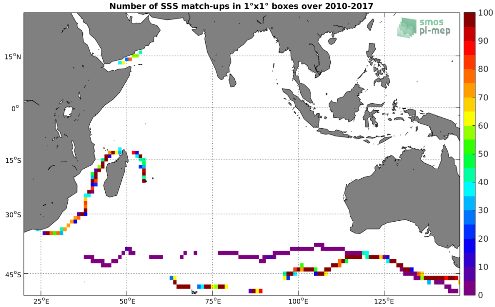
Figure 4: Number of SSS match-ups between TSG-GOSUD-Sailing-ship SSS and the SMOS-L4-CATDS-CECOS-IFREMER-V2-WEEKLY-0.5DEG SSS product for the Indian Ocean Pi-MEP region over 1^\circ \times 1^\circ boxes and for the full satellite product period.
