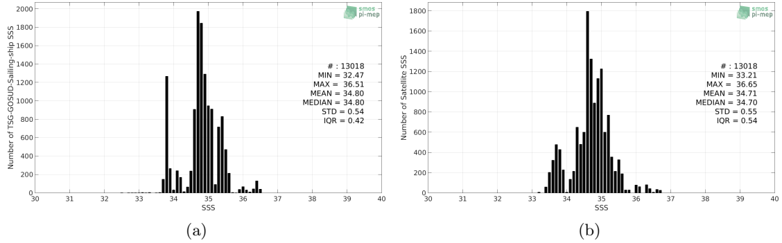
Figure 2: Histograms of SSS from TSG-GOSUD-Sailing-ship (a) and SMOS-L4-CATDS-CECOS-IFREMER-V2-WEEKLY-0.5DEG (b) considering all match-up pairs per bins of 0.1 over the Indian Ocean Pi-MEP region and for the full satellite product period.
