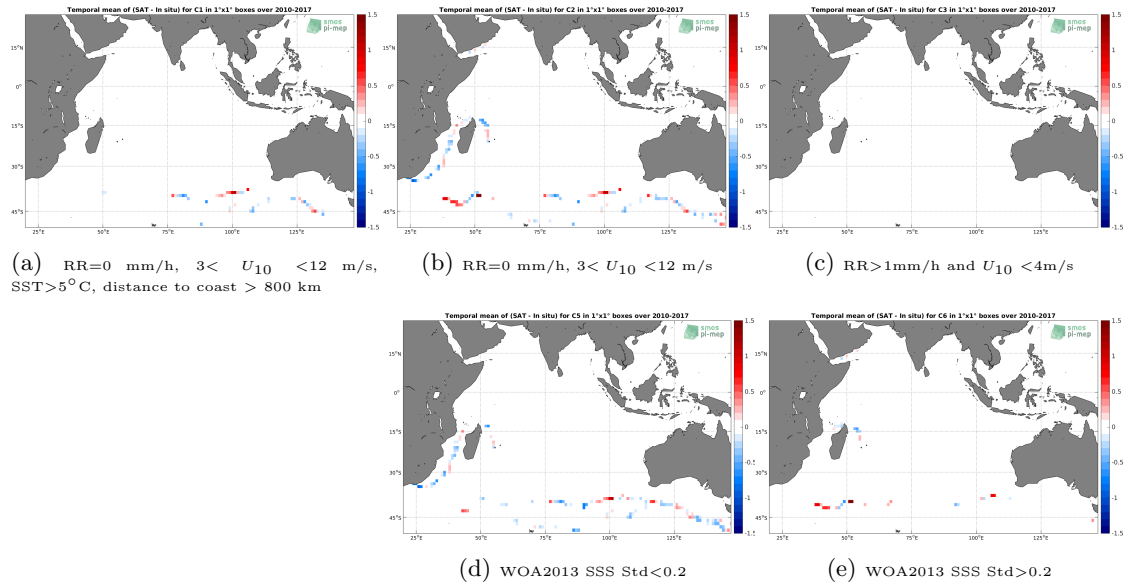
Figure 12: Temporal mean gridded over spatial boxes of size 1^\circ \times 1^\circ of \Delta SSS (SMOS-L4-CATDS-CECOS-IFREMER-V2-WEEKLY-0.5DEG - TSG-GOSUD-Sailing-ship) for 5 different subdatasets corresponding to: RR=0 mm/h, 3 < U_{10} < 12 m/s, SST > 5^\circ\text{C} , distance to coast > 800 km (a), RR=0 mm/h, 3 < U_{10} < 12 m/s (b), RR > 1 mm/h and U_{10} < 4 m/s (c), WOA2013 SSS Std < 0.2 (d), WOA2013 SSS Std > 0.2 (e).
