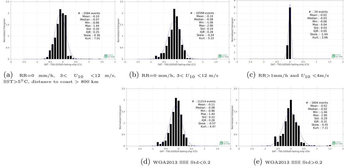
Figure 13: Normalized histogram of \Delta SSS (SMOS-L4-CATDS-CECOS-IFREMER-V2-WEEKLY-0.5DEG - TSG-GOSUD-Sailing-ship) for 5 different subdatasets corresponding to: RR=0 mm/h, 3 < U_{10} < 12 m/s, SST>5°C, distance to coast > 800 km (a), RR=0 mm/h, 3 < U_{10} < 12 m/s (b), RR>1mm/h and U_{10} < 4 m/s (c), WOA2013 SSS Std<0.2 (d), WOA2013 SSS Std>0.2 (e).
