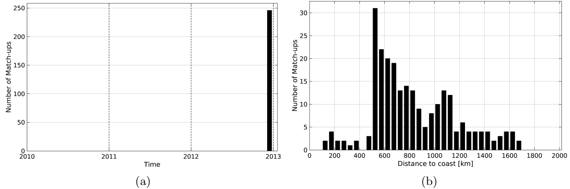
Figure 1: Number of match-ups between TSG-GOSUD-Sailing-ship and SMOS-L4-CATDS-CECOS-IFREMER-V2-WEEKLY-0.5DEG SSS as a function of time (a) and as function of the distance to coast (b) over the Indian Ocean Pi-MEP region and for the full satellite product period.
