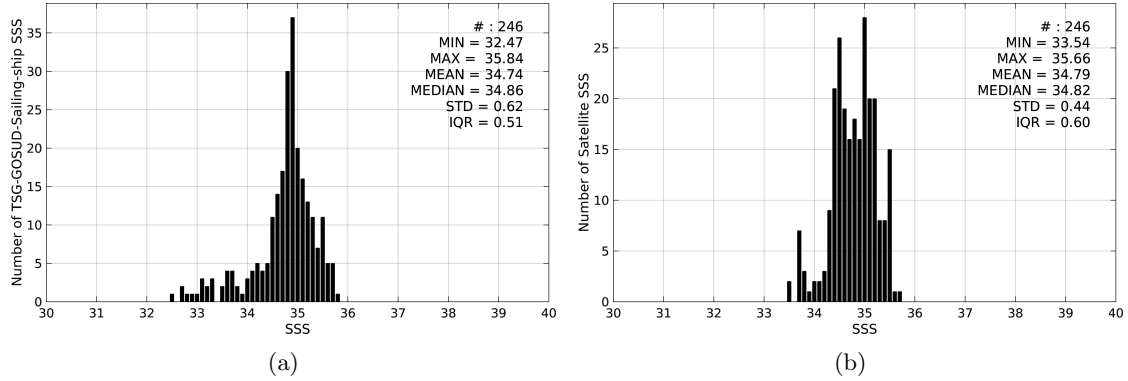
Figure 2: Histograms of SSS from TSG-GOSUD-Sailing-ship (a) and SMOS-L4-CATDS-CECOS-IFREMER-V2-WEEKLY-0.5DEG (b) considering all match-up pairs per bins of 0.1 over the Indian Ocean Pi-MEP region and for the full satellite product period.
