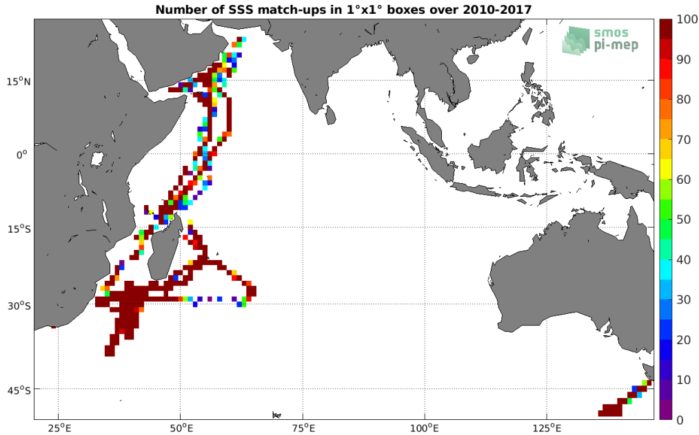
Figure 4: Number of SSS match-ups between TSG (GOSUD-Research-vessel) SSS and the SMOS L4 v2 Weekly (CATDS-CECOS-IFREMER) SSS product for the Indian Ocean Pi-MEP region over 1°x1° boxes and for the full satellite product period.
