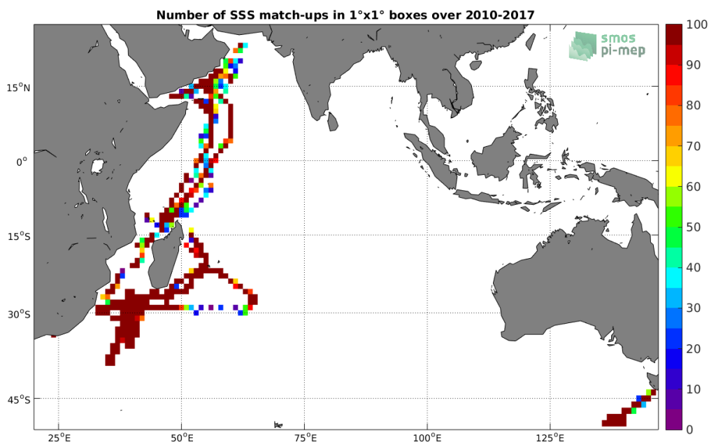
Figure 4: Number of SSS match-ups between TSG-GOSUD-Research-vessel SSS and the SMOS-L4-CATDS-CECOS-IFREMER-V2-WEEKLY-0.5DEG SSS product for the Indian Ocean Pi-MEP region over 1°x1° boxes and for the full satellite product period.
