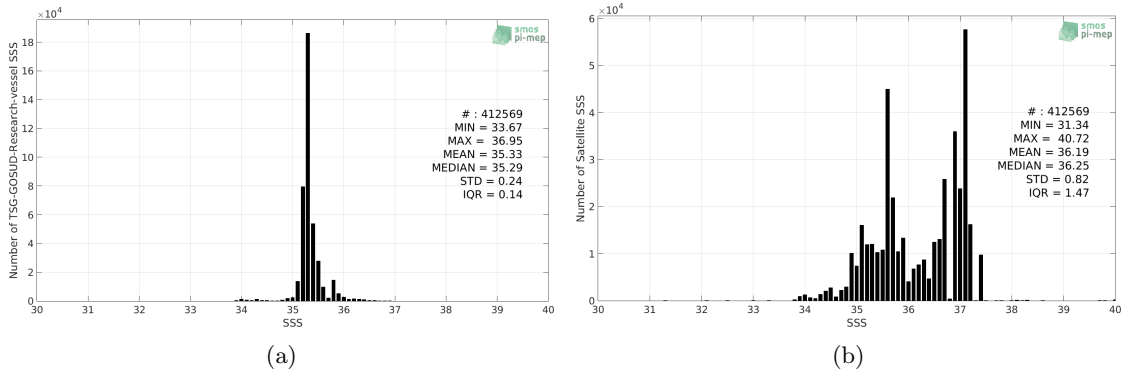
Figure 2: Histograms of SSS from TSG-GOSUD-Research-vessel (a) and SMOS-L4-CATDS-CECOS-IFREMER-V2-WEEKLY-0.5DEG (b) considering all match-up pairs per bins of 0.1 over the Indian Ocean Pi-MEP region and for the full satellite product period.
