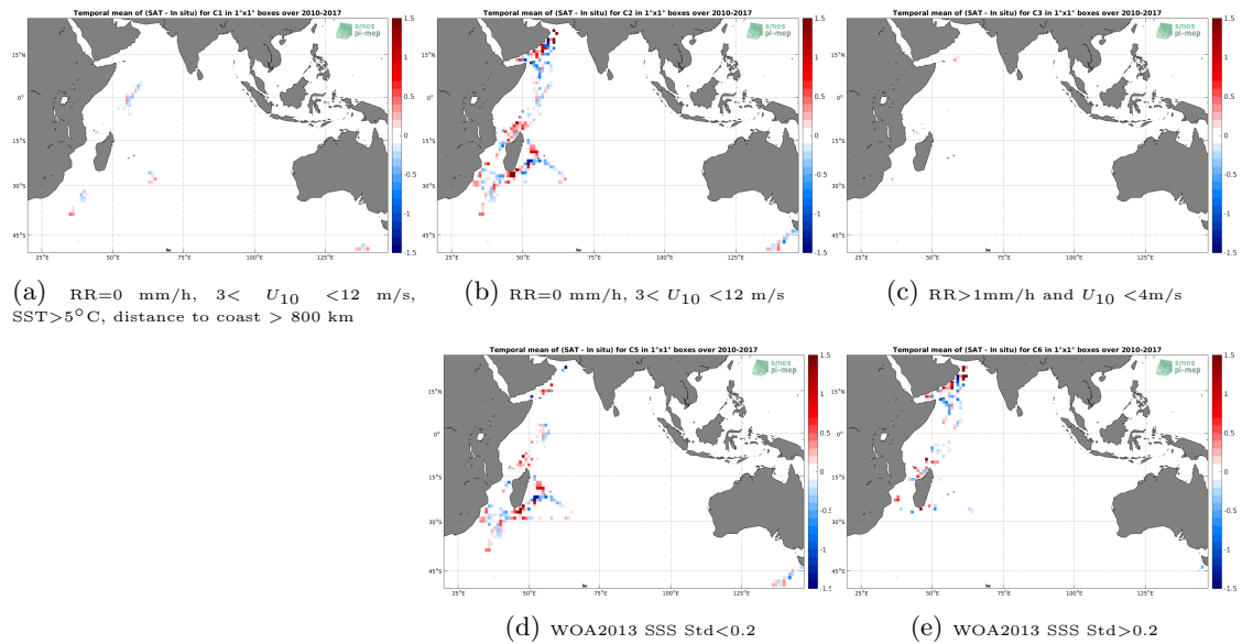
Figure 12: Temporal mean gridded over spatial boxes of size 1^\circ \times 1^\circ of \Delta SSS (SMOS-L4-CATDS-CECOS-IFREMER-V2-WEEKLY-0.5DEG - TSG-GOSUD-Research-vessel) for 5 different sub-datasets corresponding to:RR=0 mm/h, 3 < U_{10} < 12 m/s, SST >5^\circ C, distance to coast > 800 km (a), RR=0 mm/h, 3 < U_{10} < 12 m/s (b), RR >1 mm/h and U_{10} < 4 m/s (c), WOA2013 SSS Std <0.2 (d), WOA2013 SSS Std >0.2 (e).
