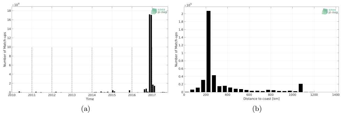
Figure 1: Number of match-ups between TSG-GOSUD-Research-vessel and SMOS-L4-CATDS-CECOS-IFREMER-V2-WEEKLY-0.5DEG SSS as a function of time (a) and as function of the distance to coast (b) over the Indian Ocean Pi-MEP region and for the full satellite product period.
