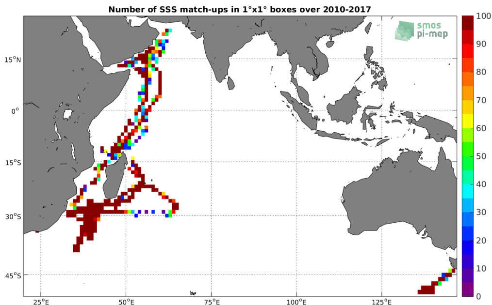
Figure 4: Number of SSS match-ups between TSG-GOSUD-Research-vessel SSS and the SMOS-L4-CATDS-CECOS-IFREMER-V2-WEEKLY-0.5DEG SSS product for the Indian Ocean Pi-MEP region over 1°x1° boxes and for the full satellite product period.
