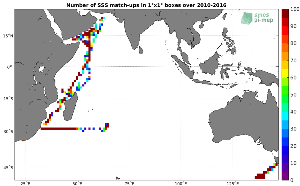
Figure 4: Number of SSS match-ups between TSG-GOSUD-Research-vessel SSS and the SMOS-L4-CATDS-CECOS-IFREMER-V2-WEEKLY-0.5DEG SSS product for the Indian Ocean Pi-MEP region over 1^\circ \times 1^\circ boxes and for the full satellite product period.
