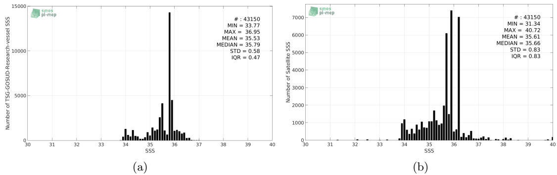
Figure 2: Histograms of SSS from TSG-GOSUD-Research-vessel (a) and SMOS-L4-CATDS-CECOS-IFREMER-V2-WEEKLY-0.5DEG (b) considering all match-up pairs per bins of 0.1 over the Indian Ocean Pi-MEP region and for the full satellite product period.
