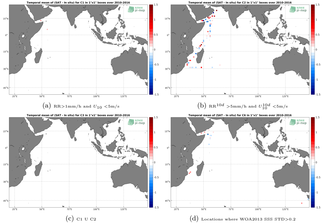
Figure 12: Temporal mean gridded over spatial boxes of size 1^\circ \times 1^\circ of \Delta SSS (SMOS-L4-CATDS-CECOS-IFREMER-V2-WEEKLY-0.5DEG - TSG-GOSUD-Research-vessel) for 4 different sub-datasets corresponding to: RR > 1mm/h and U_{10} < 5\text{m/s} (a), RR^{10d} > 5\text{mm/h} and U_{10}^{10d} < 5\text{m/s} (b), C1 U C2 (c), Locations where WOA2013 SSS STD > 0.2 (d).
