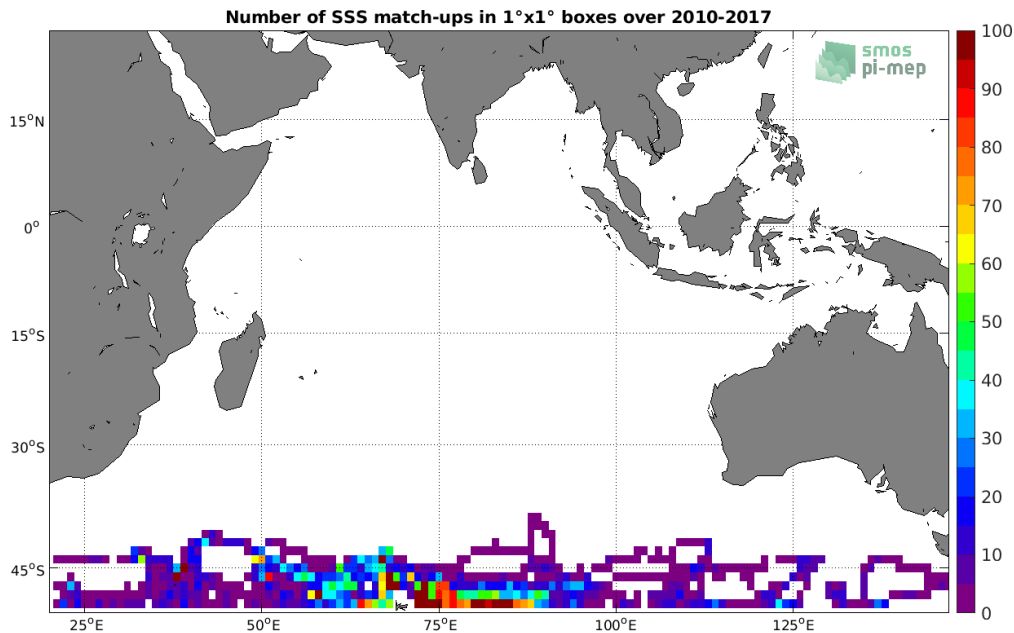
Figure 4: Number of SSS match-ups between Sea mammals SSS and the SMOS L4 v2 Weekly (CATDS-CECOS-IFREMER) SSS product for the Indian Ocean Pi-MEP region over 1^\circ \times 1^\circ boxes and for the full satellite product period.
