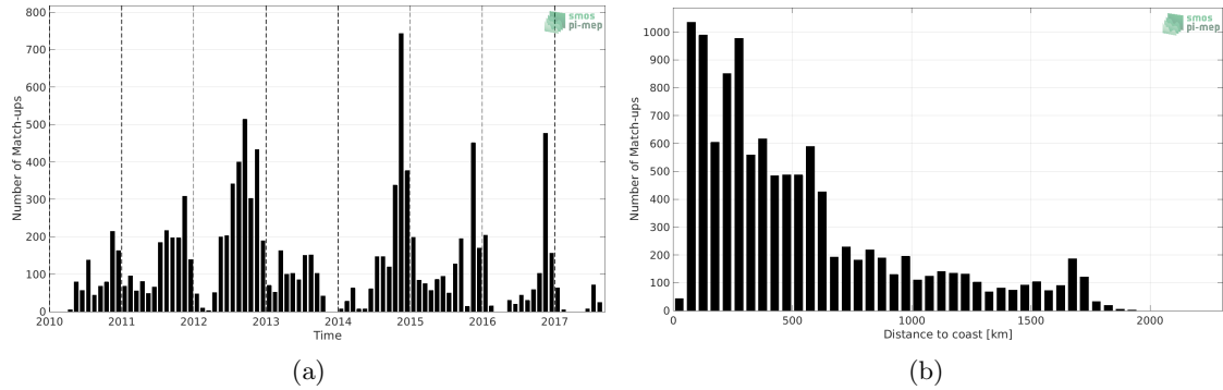
Figure 1: Number of match-ups between Sea mammals and SMOS L4 v2 Weekly (CATDS-CECOS-IFREMER) SSS as a function of time (a) and as function of the distance to coast (b) over the Indian Ocean Pi-MEP region and for the full satellite product period.
