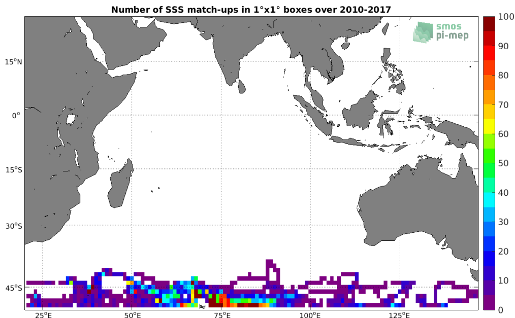
Figure 4: Number of SSS match-ups between Sea mammals SSS and the SMOS L4 v2 Weekly (CATDS-CECOS-IFREMER) SSS product for the Indian Ocean Pi-MEP region over 1°x1° boxes and for the full satellite product period.
