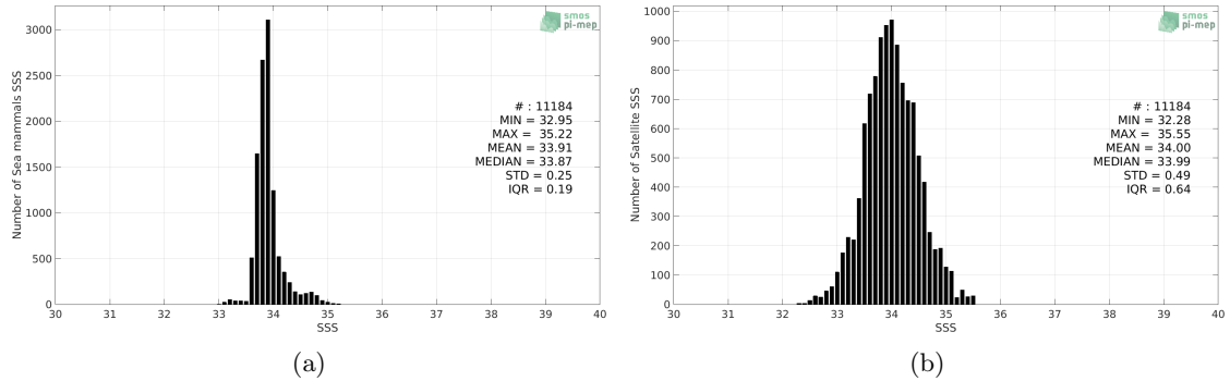
Figure 2: Histograms of SSS from Sea mammals (a) and SMOS L4 v2 Weekly (CATDS-CECOS-IFREMER) (b) considering all match-up pairs per bins of 0.1 over the Indian Ocean Pi-MEP region and for the full satellite product period.
