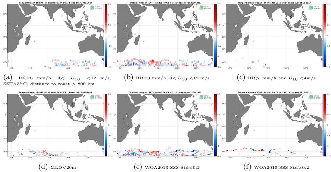
Figure 12: Temporal mean gridded over spatial boxes of size 1^{\circ}\times 1^{\circ} of \Delta\text{SSS} (SMOS L4 v2 Weekly (CATDS-CECOS-IFREMER) - Sea mammals) for 6 different subdatasets corresponding to:RR=0 mm/h, 3 < U_{10} < 12 m/s, SST >5^{\circ}\text{C} , distance to coast > 800 km (a), RR=0 mm/h, 3 < U_{10} < 12 m/s (b), RR >1 mm/h and U_{10} < 4 m/s (c),MLD <20 m (d),WOA2013 SSS Std <0.2 (e),WOA2013 SSS Std >0.2 (f).
