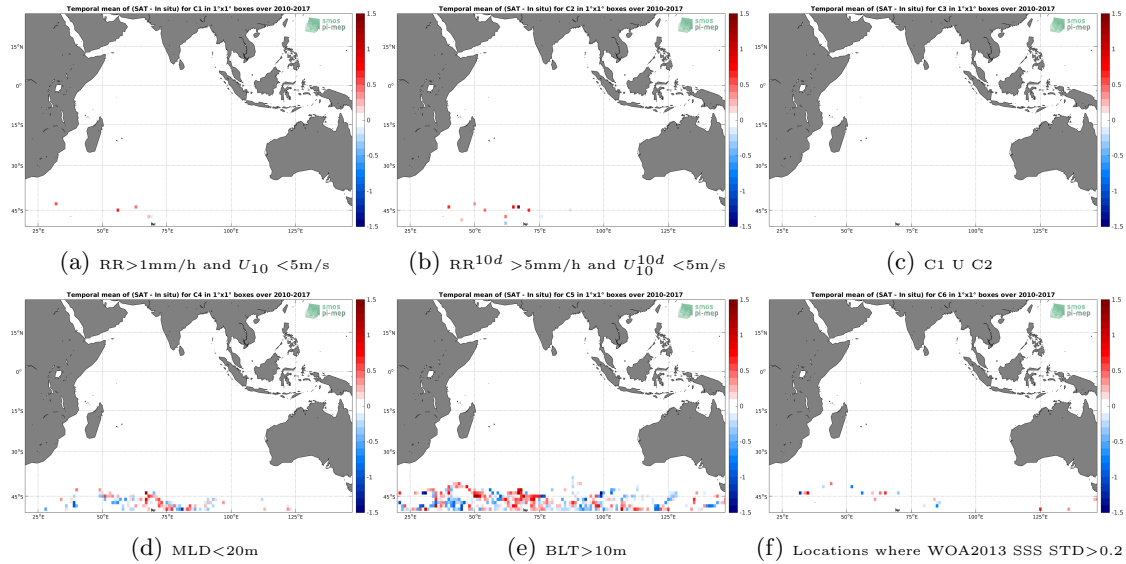
Figure 12: Temporal mean gridded over spatial boxes of size 1^\circ \times 1^\circ of \Delta\text{SSS} (SMOS-L4-CATDS-CECOS-IFREMER-V2-WEEKLY-0.5DEG - Sea mammals) for 6 different subdatasets corresponding to: \text{RR} > 1\text{mm/h} and U_{10} < 5\text{m/s} (a), \text{RR}^{10d} > 5\text{mm/h} and U_{10}^{10d} < 5\text{m/s} (b), C1 U C2 (c), \text{MLD} < 20\text{m} (d), \text{BLT} > 10\text{m} (e), Locations where WOA2013 SSS STD > 0.2 (f).
