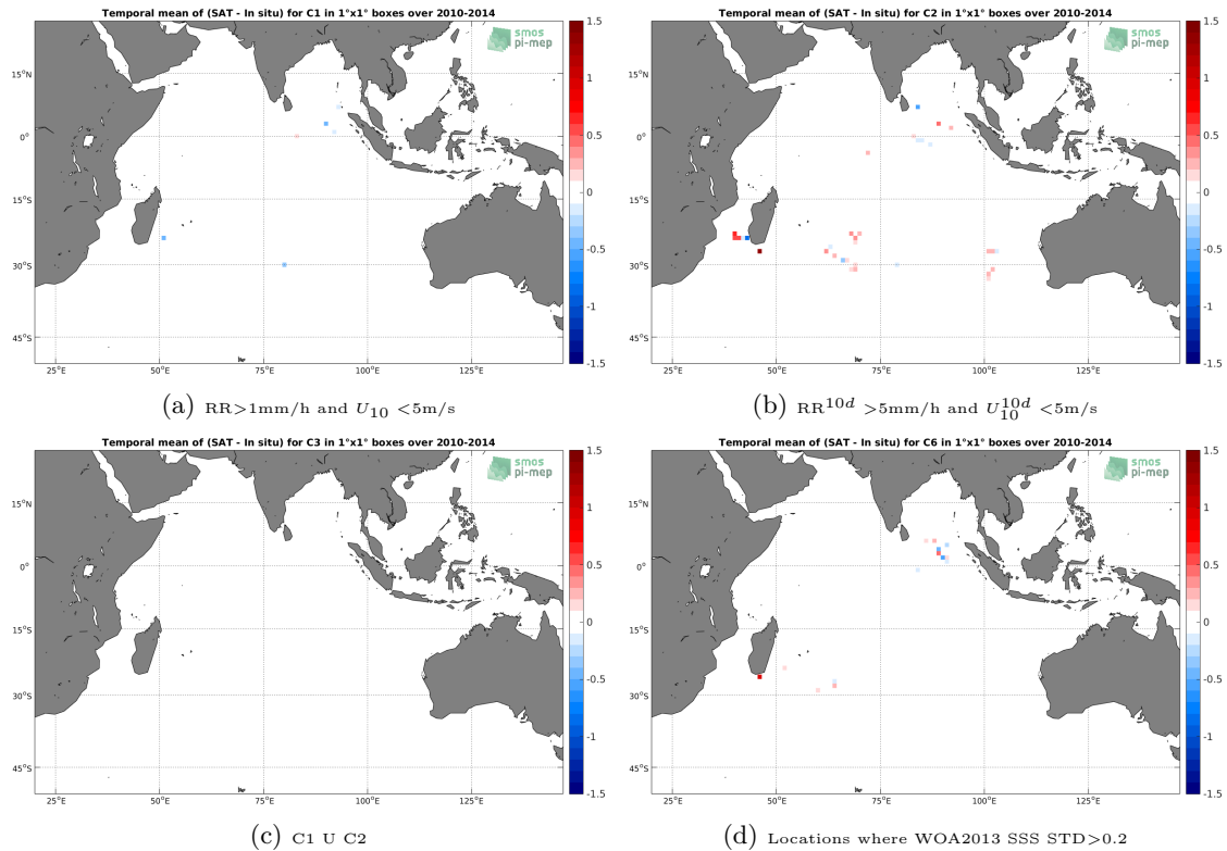
Figure 11: Temporal mean gridded over spatial boxes of size 1^\circ \times 1^\circ of \Delta SSS (SMOS-L4-CATDS-CECOS-IFREMER-V2-WEEKLY-0.5DEG - Surface drifters) for 4 different subdatasets corresponding to: RR > 1mm/h and U_{10} < 5\text{m/s} (a), RR^{10d} > 5\text{mm/h} and U_{10}^{10d} < 5\text{m/s} (b), C1 U C2 (c), Locations where WOA2013 SSS STD > 0.2 (d).
