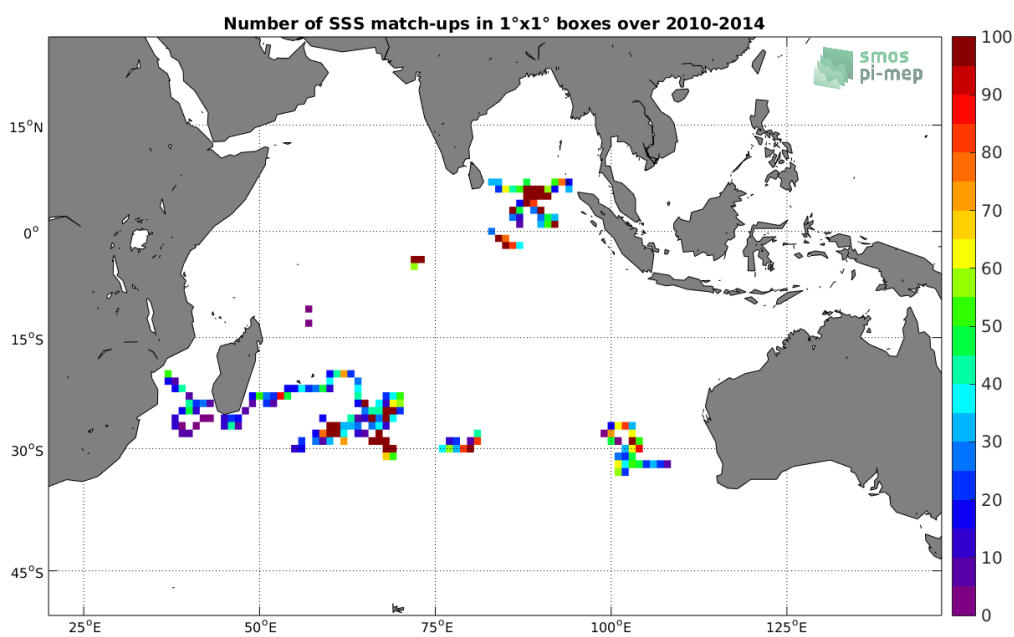
Figure 3: Number of SSS match-ups between Surface drifters SSS and the SMOS-L4-CATDS-CECOS-IFREMER-V2-WEEKLY-0.5DEG SSS product for the Indian Ocean Pi-MEP region over 1°x1° boxes and for the full satellite product period.
