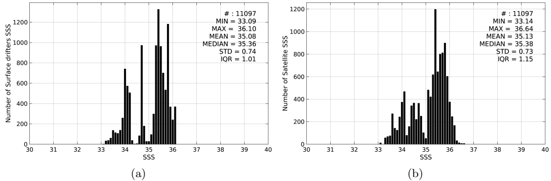
Figure 2: Histograms of SSS from Surface drifters (a) and SMOS-L4-CATDS-CECOS-IFREMER-V2-WEEKLY-0.5DEG (b) considering all match-up pairs per bins of 0.1 over the Indian Ocean Pi-MEP region and for the full satellite product period.
