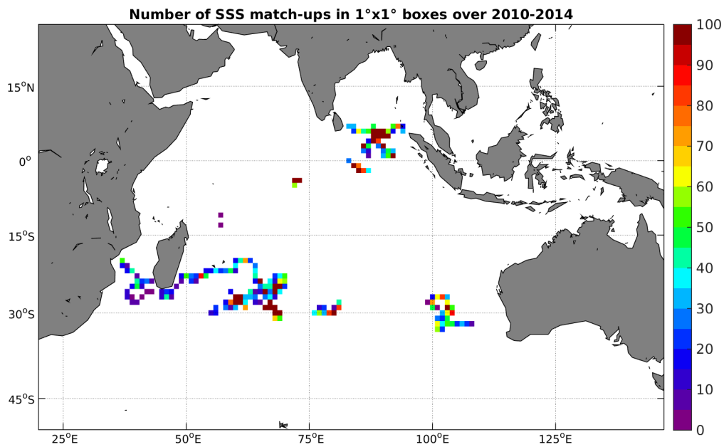
Figure 3: Number of SSS match-ups between Surface drifters SSS and the SMOS-L4-CATDS-CECOS-IFREMER-V2-WEEKLY-0.5DEG SSS product for the Indian Ocean Pi-MEP region over 1°x1° boxes and for the full satellite product period.
