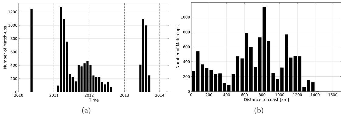
Figure 1: Number of match-ups between Surface drifters and SMOS-L4-CATDS-CECOS-IFREMER-V2-WEEKLY-0.5DEG SSS as a function of time (a) and as function of the distance to coast (b) over the Indian Ocean Pi-MEP region and for the full satellite product period.
