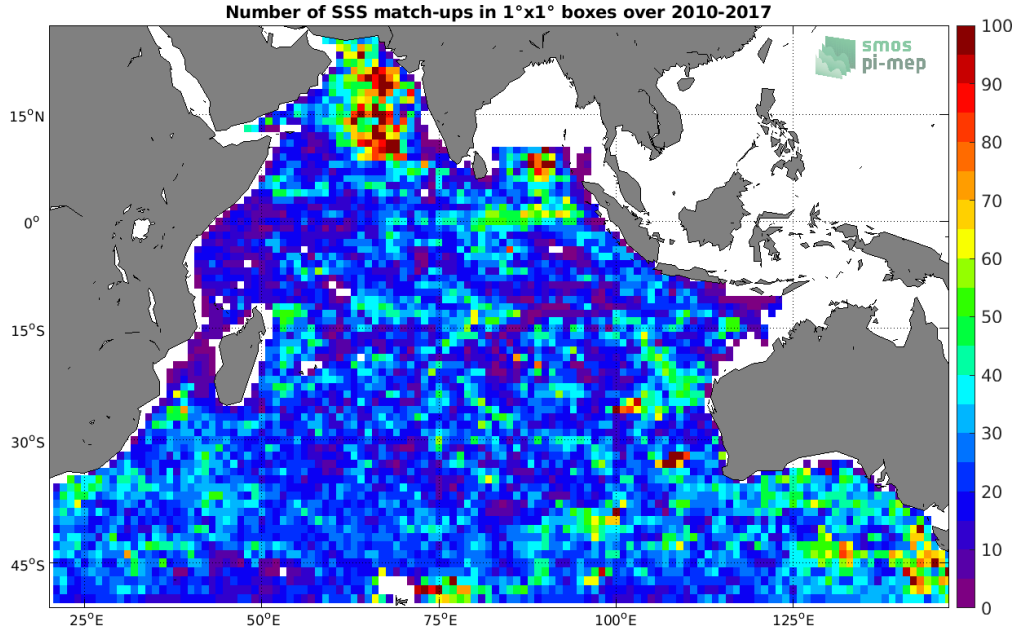
Figure 4: Number of SSS match-ups between Argo SSS and the SMOS L4 v2 Weekly (CATDS-CECOS-IFREMER) SSS product for the Indian Ocean Pi-MEP region over 1^\circ \times 1^\circ boxes and for the full satellite product period.
