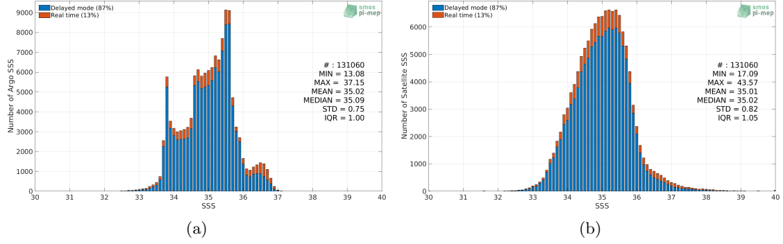
Figure 2: Histograms of SSS from Argo (a) and SMOS L4 v2 Weekly (CATDS-CECOS-IFREMER) (b) considering all match-up pairs per bins of 0.1 over the Indian Ocean Pi-MEP region and for the full satellite product period.
