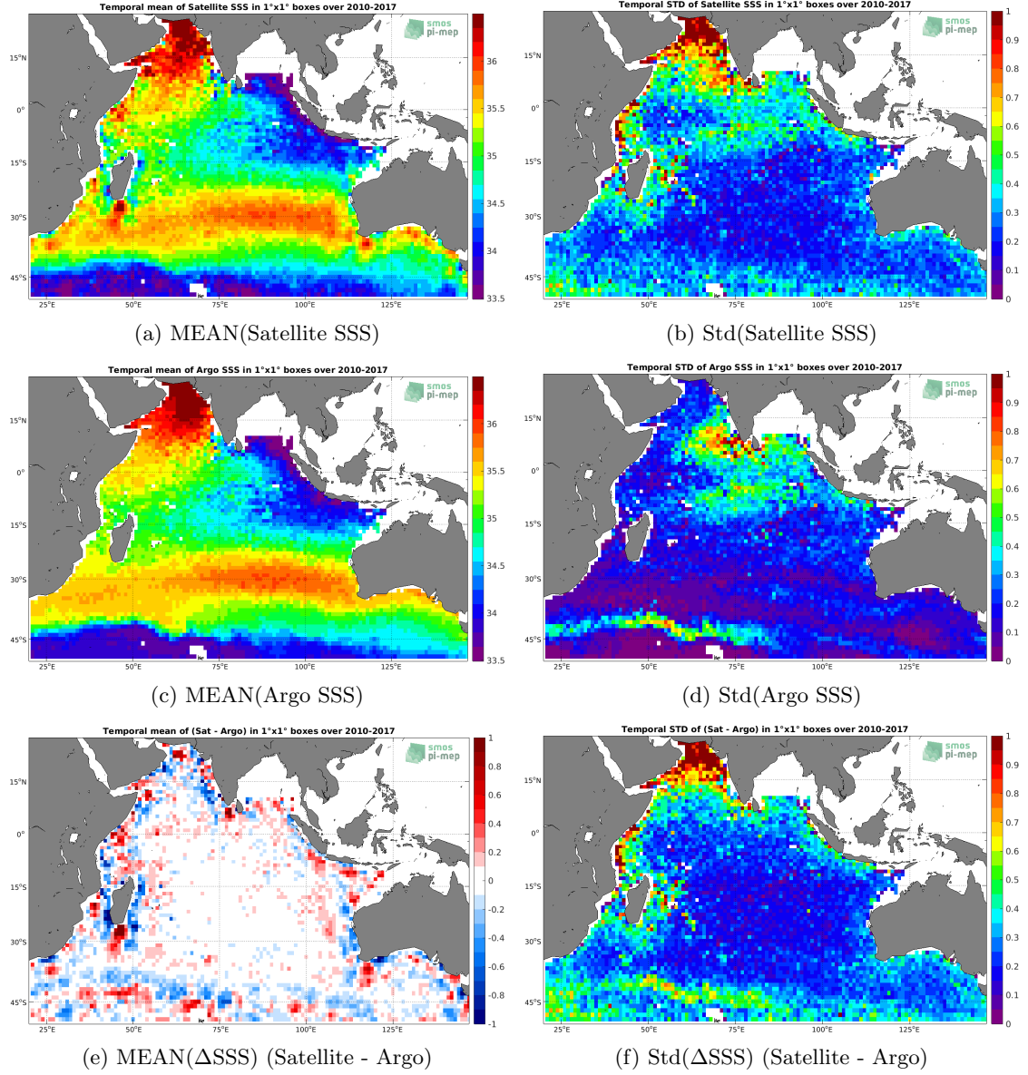
Figure 6: Temporal mean (left) and Std (right) of SSS from SMOS L4 v2 Weekly (CATDS-CECOS-IFREMER) (top), Argo (middle), and of \Delta SSS (Satellite - Argo). Only match-up pairs are used to generate these maps.
