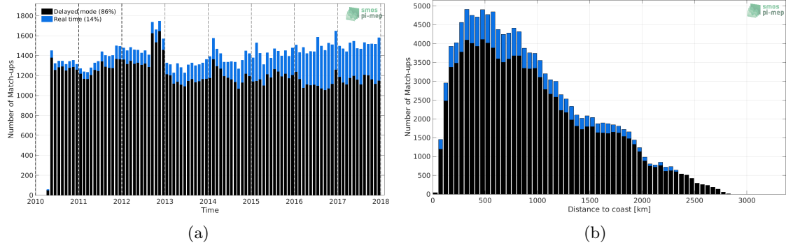
Figure 1: Number of match-ups between Argo and SMOS L4 v2 Weekly (CATDS-CECOS-IFREMER) SSS as a function of time (a) and as function of the distance to coast (b) over the Indian Ocean Pi-MEP region and for the full satellite product period.
