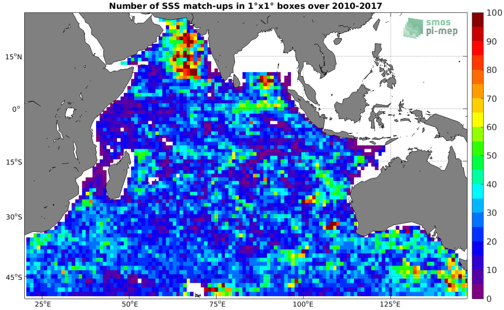
Figure 4: Number of SSS match-ups between Argo SSS and the SMOS L4 v2 Weekly (CATDS-CECOS-IFREMER) SSS product for the Indian Ocean Pi-MEP region over 1^\circ \times 1^\circ boxes and for the full satellite product period.
