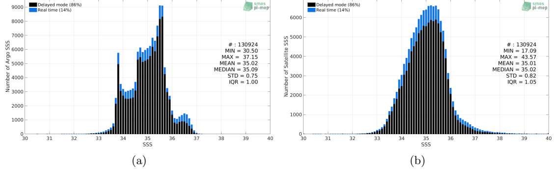
Figure 2: Histograms of SSS from Argo (a) and SMOS L4 v2 Weekly (CATDS-CECOS-IFREMER) (b) considering all match-up pairs per bins of 0.1 over the Indian Ocean Pi-MEP region and for the full satellite product period.
