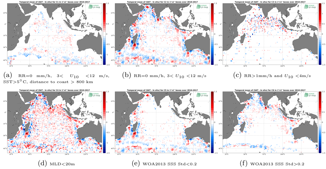
Figure 12: Temporal mean gridded over spatial boxes of size 1^\circ \times 1^\circ of \Delta SSS (SMOS-L4-CATDS-CECOS-IFREMER-V2-WEEKLY-0.5DEG - Argo) for 6 different subdatasets corresponding to: RR=0 mm/h, 3 < U_{10} < 12 m/s, SST > 5^\circ C , distance to coast > 800 km (a), RR=0 mm/h, 3 < U_{10} < 12 m/s (b), RR > 1 mm/h and U_{10} < 4 m/s (c), MLD < 20 m (d), WOA2013 SSS Std < 0.2 (e), WOA2013 SSS Std > 0.2 (f).
