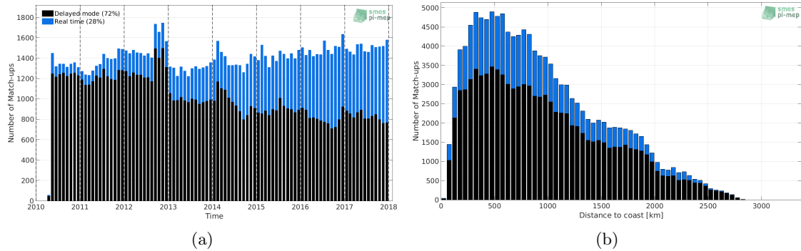
Figure 1: Number of match-ups between Argo and SMOS-L4-CATDS-CECOS-IFREMER-V2-WEEKLY-0.5DEG SSS as a function of time (a) and as function of the distance to coast (b) over the Indian Ocean Pi-MEP region and for the full satellite product period.
