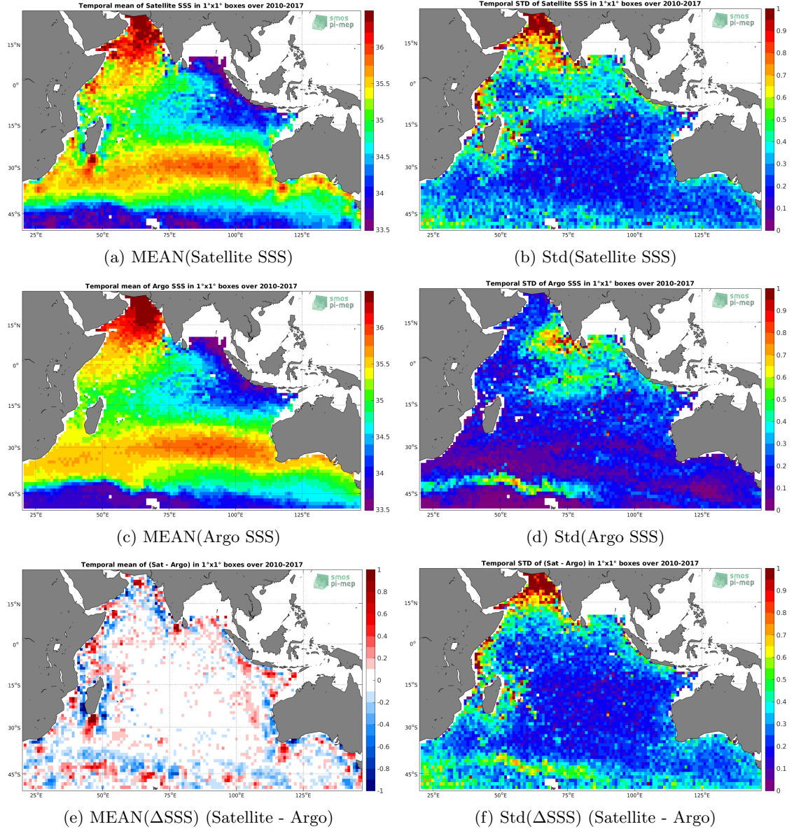
Figure 6: Temporal mean (left) and Std (right) of SSS from SMOS-L4-CATDS-CECOS-IFREMER-V2-WEEKLY-0.5DEG (top), Argo (middle), and of \Delta SSS (Satellite - Argo). Only match-up pairs are used to generate these maps.
