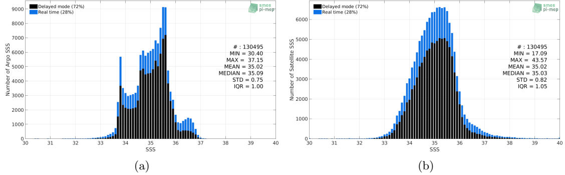
Figure 2: Histograms of SSS from Argo (a) and SMOS-L4-CATDS-CECOS-IFREMER-V2-WEEKLY-0.5DEG (b) considering all match-up pairs per bins of 0.1 over the Indian Ocean Pi-MEP region and for the full satellite product period.
