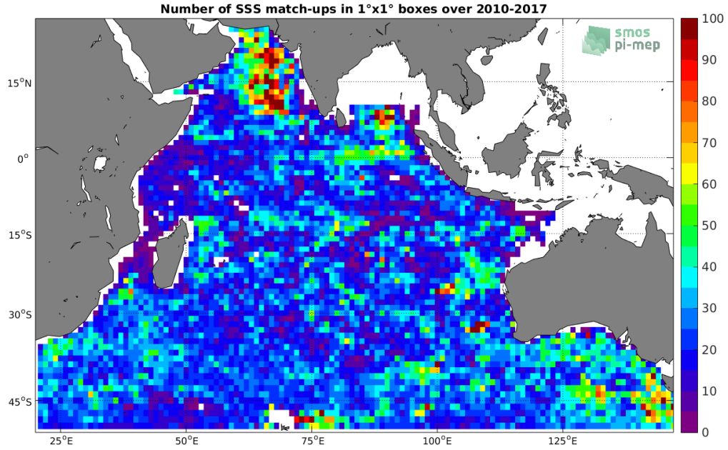
Figure 4: Number of SSS match-ups between Argo SSS and the SMOS-L4-CATDS-CECOS-IFREMER-V2-WEEKLY-0.5DEG SSS product for the Indian Ocean Pi-MEP region over 1^\circ \times 1^\circ boxes and for the full satellite product period.
