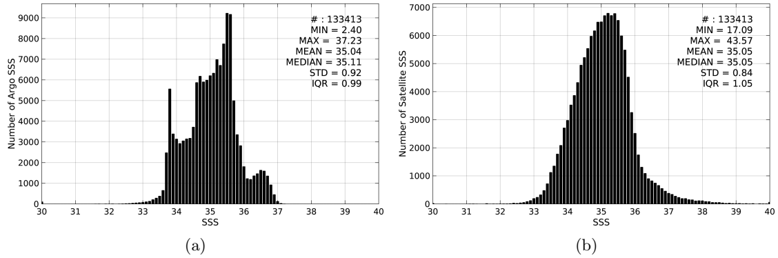
Figure 2: Histograms of SSS from Argo (a) and SMOS-L4-CATDS-CECOS-IFREMER-V2-WEEKLY-0.5DEG (b) considering all match-up pairs per bins of 0.1 over the Indian Ocean Pi-MEP region and for the full satellite product period.
