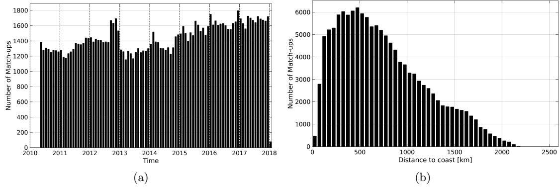
Figure 1: Number of match-ups between Argo and SMOS-L4-CATDS-CECOS-IFREMER-V2-WEEKLY-0.5DEG SSS as a function of time (a) and as function of the distance to coast (b) over the Indian Ocean Pi-MEP region and for the full satellite product period.
