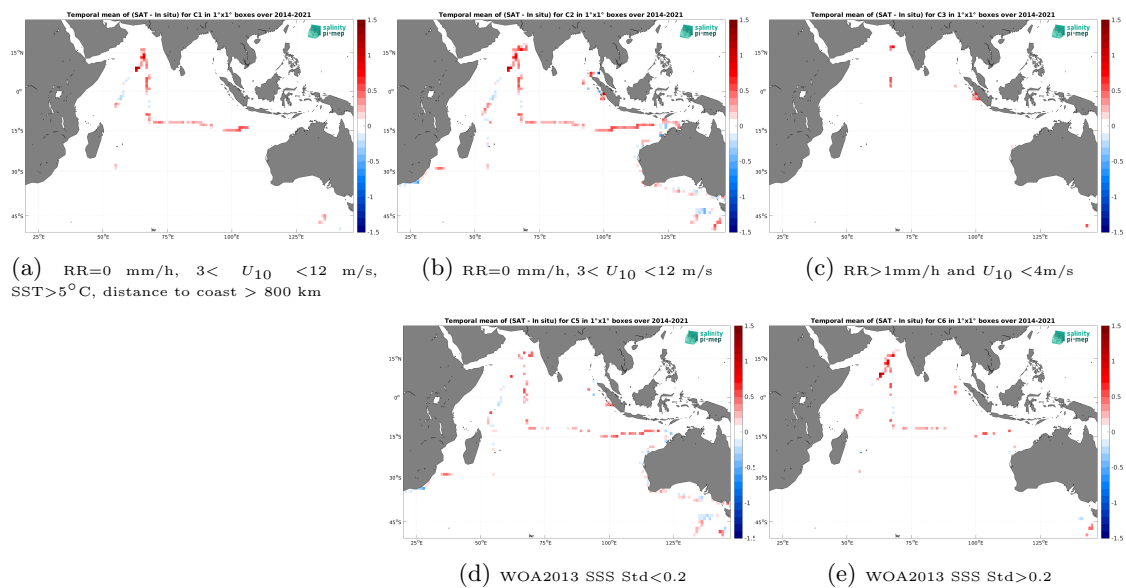
Figure 14: Temporal mean gridded over spatial boxes of size 1^\circ \times 1^\circ of \Delta SSS (SMOS SSS L4 v2 - Daily (BEC) - TSG (SAMOS)) for 5 different subdatasets corresponding to:RR=0 mm/h, 3 < U_{10} < 12 m/s, SST >5^\circ\text{C} , distance to coast > 800 km (a), RR=0 mm/h, 3 < U_{10} < 12 m/s (b), RR >1 mm/h and U_{10} < 4 m/s (c), WOA2013 SSS Std <0.2 (d), WOA2013 SSS Std >0.2 (e).
