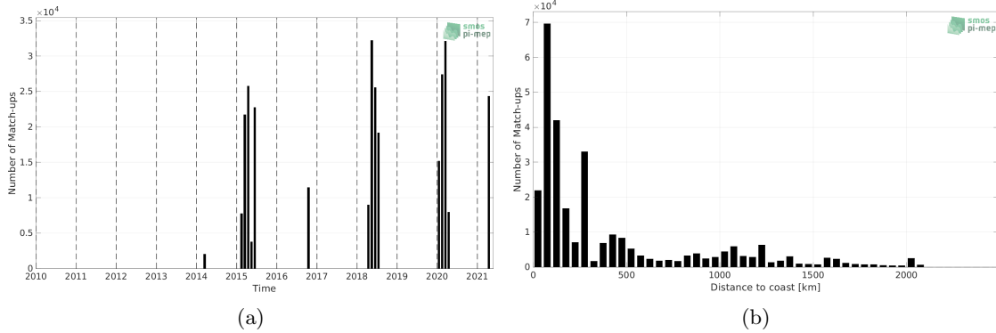
Figure 1: Number of match-ups between TSG (SAMOS) and SMOS SSS L4 v2 - Daily (BEC) SSS as a function of time (a) and as function of the distance to coast (b) over the Indian Ocean Pi-MEP region and for the full satellite product period.
