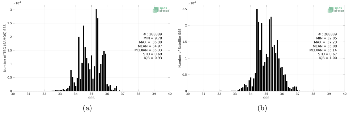
Figure 2: Histograms of SSS from TSG (SAMOS) (a) and SMOS SSS L4 v2 - Daily (BEC) (b) considering all match-up pairs per bins of 0.1 over the Indian Ocean Pi-MEP region and for the full satellite product period.
