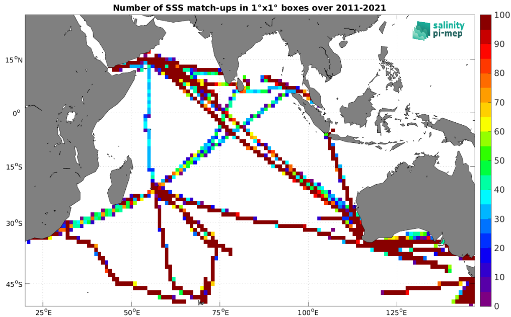
Figure 5: Number of SSS match-ups between TSG (LEGOS-DM) SSS and the SMOS SSS L4 v2 - Daily (BEC) SSS product for the Indian Ocean Pi-MEP region over 1^\circ \times 1^\circ boxes and for the full satellite product period.
