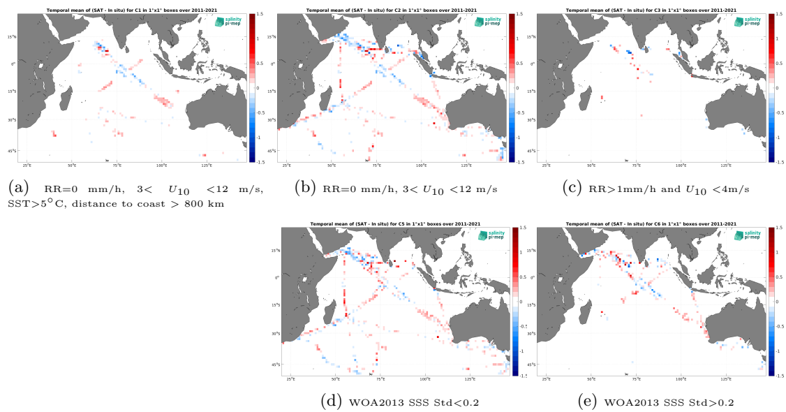
Figure 14: Temporal mean gridded over spatial boxes of size 1^\circ \times 1^\circ of \Delta\text{SSS} (SMOS SSS L4 v2 - Daily (BEC) - TSG (LEGOS-DM)) for 5 different subdatasets corresponding to:RR=0 mm/h, 3 < U_{10} < 12 m/s, SST > 5^\circ\text{C} , distance to coast > 800 km (a), RR=0 mm/h, 3 < U_{10} < 12 m/s (b), RR > 1\text{mm/h} and U_{10} < 4\text{m/s} (c), WOA2013 SSS Std < 0.2 (d), WOA2013 SSS Std > 0.2 (e).
