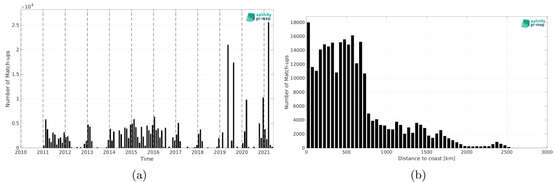
Figure 2: Number of match-ups between TSG (LEGOS-DM) and SMOS SSS L4 v2 - Daily (BEC) SSS as a function of time (a) and as function of the distance to coast (b) over the Indian Ocean Pi-MEP region and for the full satellite product period.
