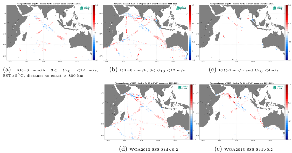
Figure 14: Temporal mean gridded over spatial boxes of size 1^\circ \times 1^\circ of \Delta SSS (SMOS SSS L4 v2 - Daily (BEC) - TSG (LEGOS-DM)) for 5 different subdatasets corresponding to:RR=0 mm/h, 3 < U_{10} < 12 m/s, SST > 5^\circ\text{C} , distance to coast > 800 km (a), RR=0 mm/h, 3 < U_{10} < 12 m/s (b), RR > 1 mm/h and U_{10} < 4 m/s (c), WOA2013 SSS Std < 0.2 (d), WOA2013 SSS Std > 0.2 (e).
