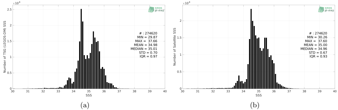
Figure 2: Histograms of SSS from TSG (LEGOS-DM) (a) and SMOS SSS L4 v2 - Daily (BEC) (b) considering all match-up pairs per bins of 0.1 over the Indian Ocean Pi-MEP region and for the full satellite product period.
