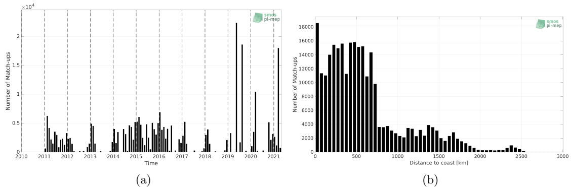
Figure 1: Number of match-ups between TSG (LEGOS-DM) and SMOS SSS L4 v2 - Daily (BEC) SSS as a function of time (a) and as function of the distance to coast (b) over the Indian Ocean Pi-MEP region and for the full satellite product period.
