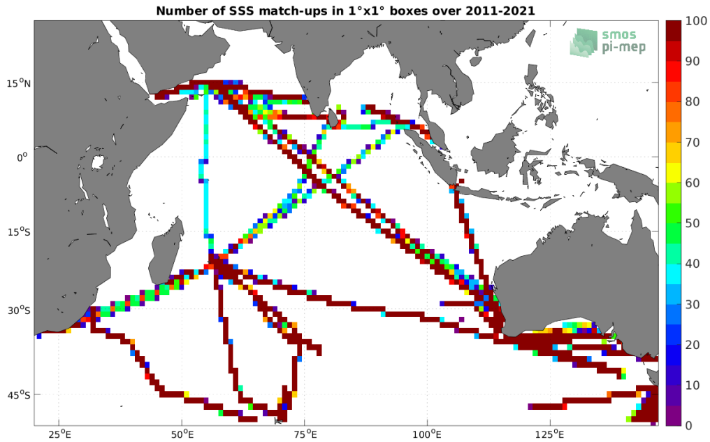
Figure 4: Number of SSS match-ups between TSG (LEGOS-DM) SSS and the SMOS SSS L4 v2 - Daily (BEC) SSS product for the Indian Ocean Pi-MEP region over 1^\circ \times 1^\circ boxes and for the full satellite product period.
