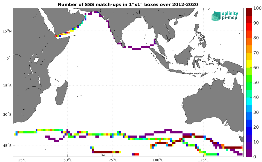
Figure 5: Number of SSS match-ups between TSG (GOSUD-Sailing-ship) SSS and the SMOS SSS L4 v2 - Daily (BEC) SSS product for the Indian Ocean Pi-MEP region over 1^\circ \times 1^\circ boxes and for the full satellite product period.
