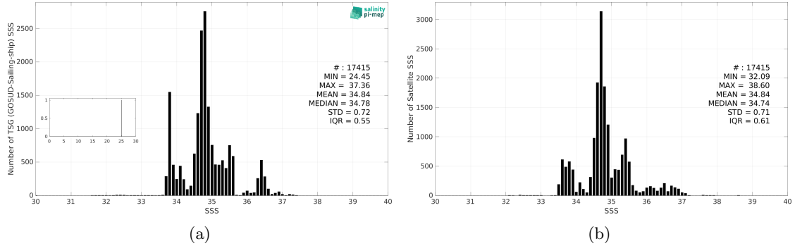
Figure 3: Histograms of SSS from TSG (GOSUD-Sailing-ship) (a) and SMOS SSS L4 v2 - Daily (BEC) (b) considering all match-up pairs per bins of 0.1 over the Indian Ocean Pi-MEP region and for the full satellite product period.
