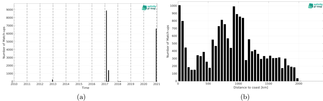
Figure 2: Number of match-ups between TSG (GOSUD-Sailing-ship) and SMOS SSS L4 v2 - Daily (BEC) SSS as a function of time (a) and as function of the distance to coast (b) over the Indian Ocean Pi-MEP region and for the full satellite product period.
