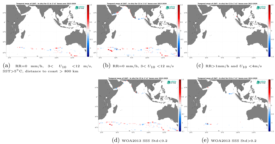
Figure 14: Temporal mean gridded over spatial boxes of size 1^\circ \times 1^\circ of \Delta SSS (SMOS SSS L4 v2 - Daily (BEC) - TSG (GOSUD-Sailing-ship)) for 5 different subdatasets corresponding to:RR=0 mm/h, 3 < U_{10} < 12 m/s, SST > 5^\circ\text{C} , distance to coast > 800 km (a), RR=0 mm/h, 3 < U_{10} < 12 m/s (b), RR > 1 mm/h and U_{10} < 4 m/s (c), WOA2013 SSS Std < 0.2 (d), WOA2013 SSS Std > 0.2 (e).
