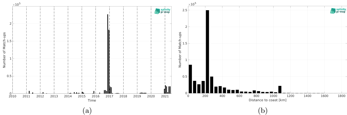
Figure 2: Number of match-ups between TSG (GOSUD-Research-vessel) and SMOS SSS L4 v2 - Daily (BEC) SSS as a function of time (a) and as function of the distance to coast (b) over the Indian Ocean Pi-MEP region and for the full satellite product period.
