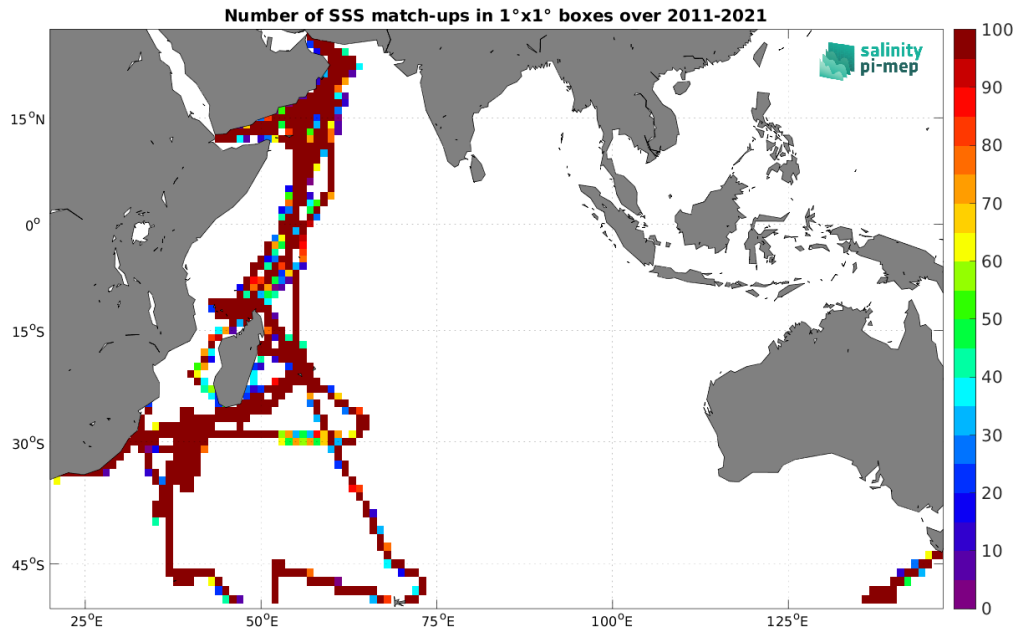
Figure 5: Number of SSS match-ups between TSG (GOSUD-Research-vessel) SSS and the SMOS SSS L4 v2 - Daily (BEC) SSS product for the Indian Ocean Pi-MEP region over 1^{\circ} \times 1^{\circ} boxes and for the full satellite product period.
