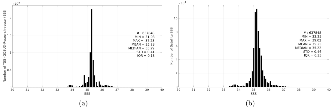
Figure 3: Histograms of SSS from TSG (GOSUD-Research-vessel) (a) and SMOS SSS L4 v2 - Daily (BEC) (b) considering all match-up pairs per bins of 0.1 over the Indian Ocean Pi-MEP region and for the full satellite product period.
