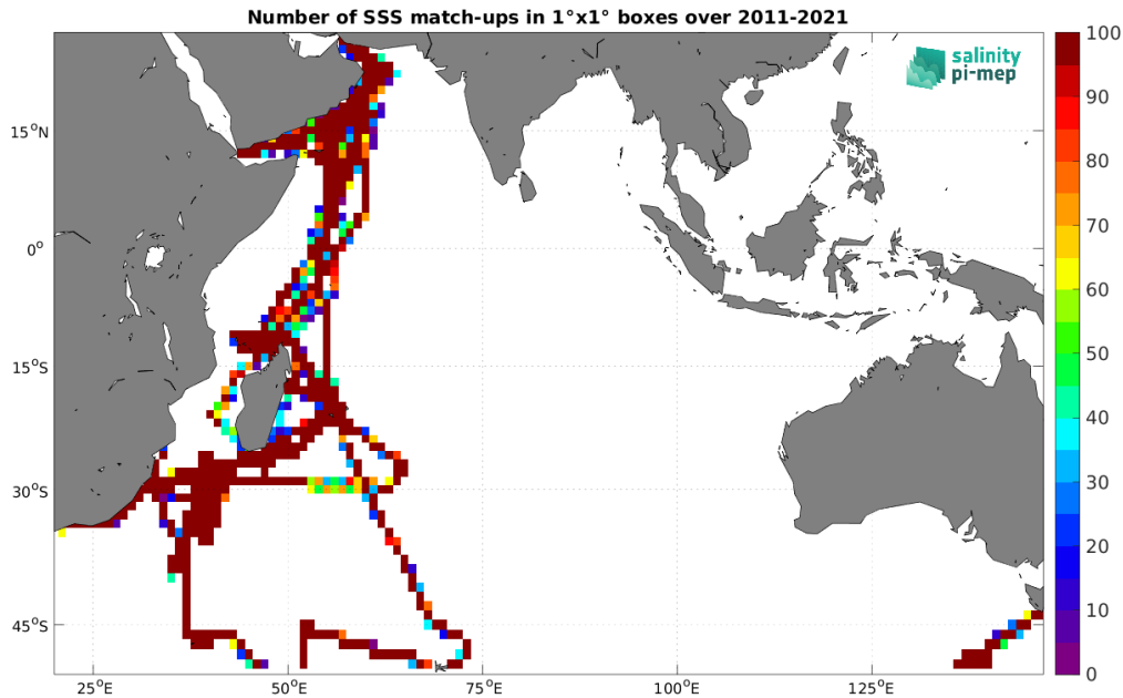
Figure 5: Number of SSS match-ups between TSG (GOSUD-Research-vessel) SSS and the SMOS SSS L4 v2 - Daily (BEC) SSS product for the Indian Ocean Pi-MEP region over 1^{\circ} \times 1^{\circ} boxes and for the full satellite product period.
