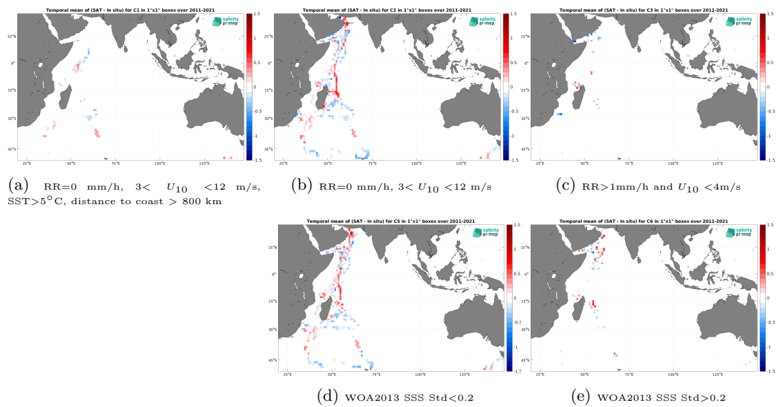
Figure 12: Temporal mean gridded over spatial boxes of size 1^\circ \times 1^\circ of \Delta SSS (SMOS SSS L4 v2 - Daily (BEC) - TSG (GOSUD-Research-vessel)) for 5 different subdatasets corresponding to:RR=0 mm/h, 3 < U_{10} < 12 m/s, SST >5^\circ C, distance to coast > 800 km (a), RR=0 mm/h, 3 < U_{10} < 12 m/s (b), RR >1 mm/h and U_{10} < 4 m/s (c), WOA2013 SSS Std <0.2 (d), WOA2013 SSS Std >0.2 (e).
