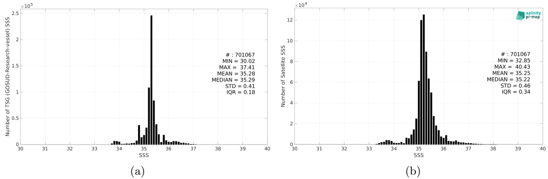
Figure 2: Histograms of SSS from TSG (GOSUD-Research-vessel) (a) and SMOS SSS L4 v2 - Daily (BEC) (b) considering all match-up pairs per bins of 0.1 over the Indian Ocean Pi-MEP region and for the full satellite product period.
