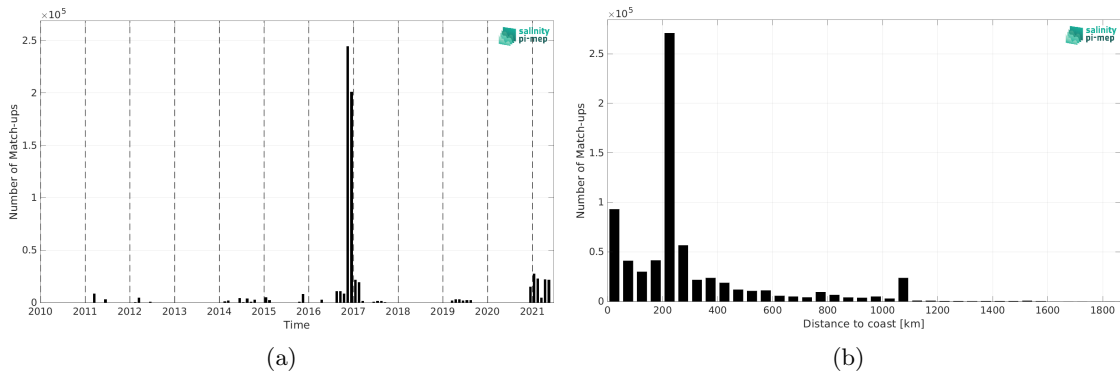
Figure 1: Number of match-ups between TSG (GOSUD-Research-vessel) and SMOS SSS L4 v2 - Daily (BEC) SSS as a function of time (a) and as function of the distance to coast (b) over the Indian Ocean Pi-MEP region and for the full satellite product period.
