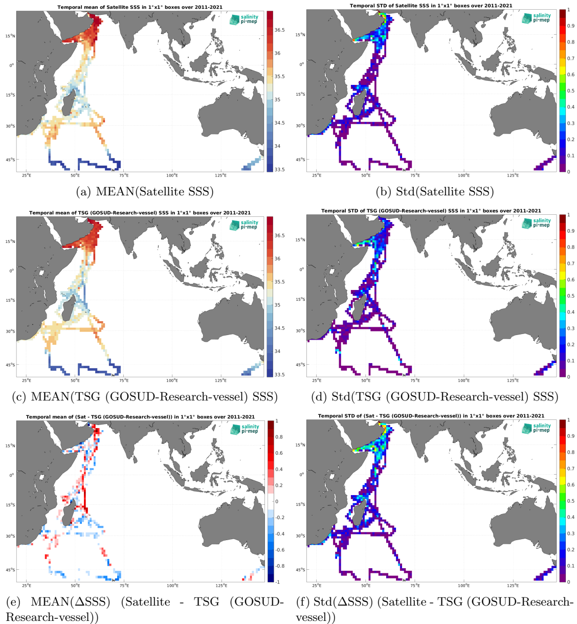
Figure 6: Temporal mean (left) and Std (right) of SSS from SMOS SSS L4 v2 - Daily (BEC) (top), TSG (GOSUD-Research-vessel) (middle), and of \Delta SSS (Satellite - TSG (GOSUD-Research-vessel)). Only match-up pairs are used to generate these maps.
