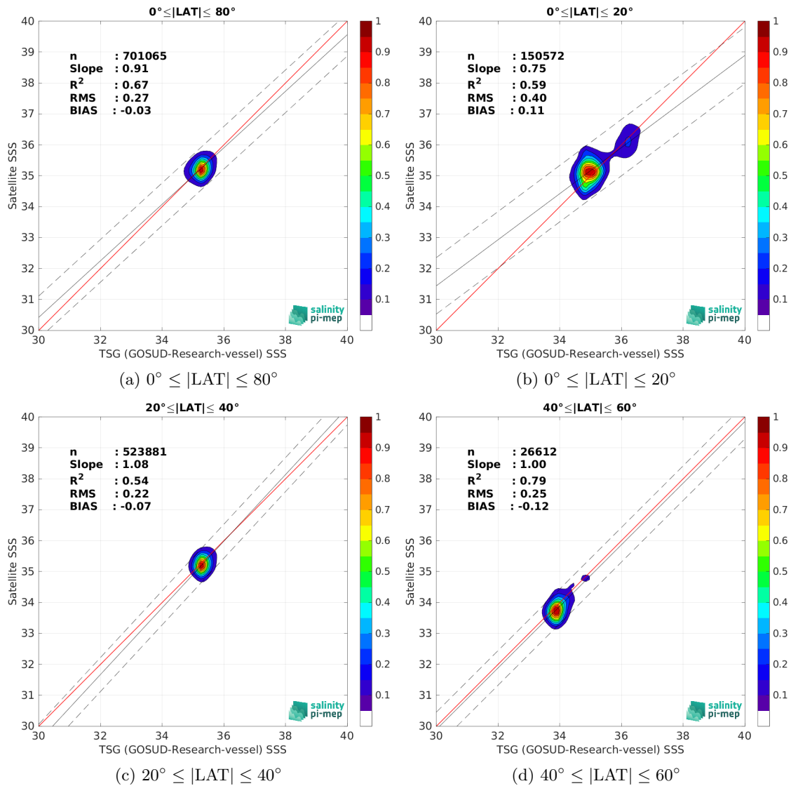
Figure 9: Contour maps of the concentration of SMOS SSS L4 v2 - Daily (BEC) SSS (y-axis) versus TSG (GOSUD-Research-vessel) SSS (x-axis) at match-up pairs for different latitude bands. For each plot, the red line shows x=y . The black thin and dashed lines indicate a linear fit through the data cloud and the \pm 95\% confidence levels, respectively. The number match-up pairs n , the slope and R^2 coefficient of the linear fit, the root mean square (RMS) and the mean bias between satellite and in situ data are indicated for each latitude band in each plots.
