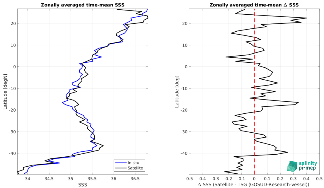
Figure 8: Left panel: Zonal mean SSS from SMOS SSS L4 v2 - Daily (BEC) satellite product (black) and from TSG (GOSUD-Research-vessel) (blue). Right panel: Zonal mean of \Delta SSS (Satellite - TSG (GOSUD-Research-vessel)) for all the collected Pi-MEP match-up pairs estimated over the full satellite product period.
