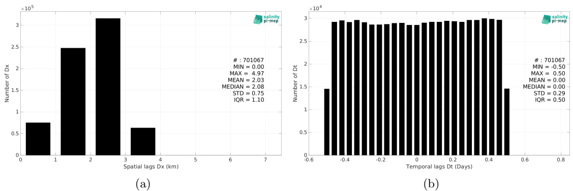
Figure 5: Histograms of the spatial (a) and temporal (b) lags between the location/time of the TSG (GOSUD-Research-vessel) measurement and the date of the corresponding SMOS SSS L4 v2 - Daily (BEC) SSS pixel.
