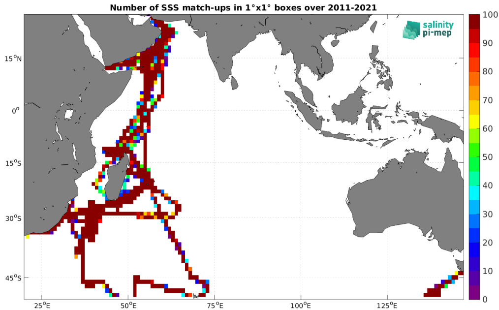
Figure 4: Number of SSS match-ups between TSG (GOSUD-Research-vessel) SSS and the SMOS SSS L4 v2 - Daily (BEC) SSS product for the Indian Ocean Pi-MEP region over 1°x1° boxes and for the full satellite product period.
