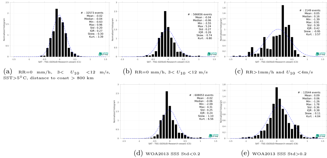
Figure 13: Normalized histogram of \Delta SSS (SMOS SSS L4 v2 - Daily (BEC) - TSG (GOSUD-Research-vessel)) for 5 different subdatasets corresponding to: RR=0 mm/h, 3 < U_{10} < 12 m/s, SST > 5°C, distance to coast > 800 km (a), RR=0 mm/h, 3 < U_{10} < 12 m/s (b), RR > 1mm/h and U_{10} < 4 m/s (c), WOA2013 SSS Std < 0.2 (d), WOA2013 SSS Std > 0.2 (e).
